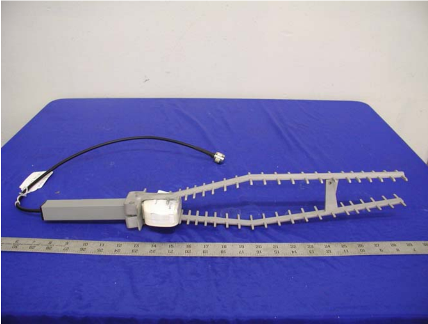
PAWVA24-16, 16dB Vagi Antenna – Side View
