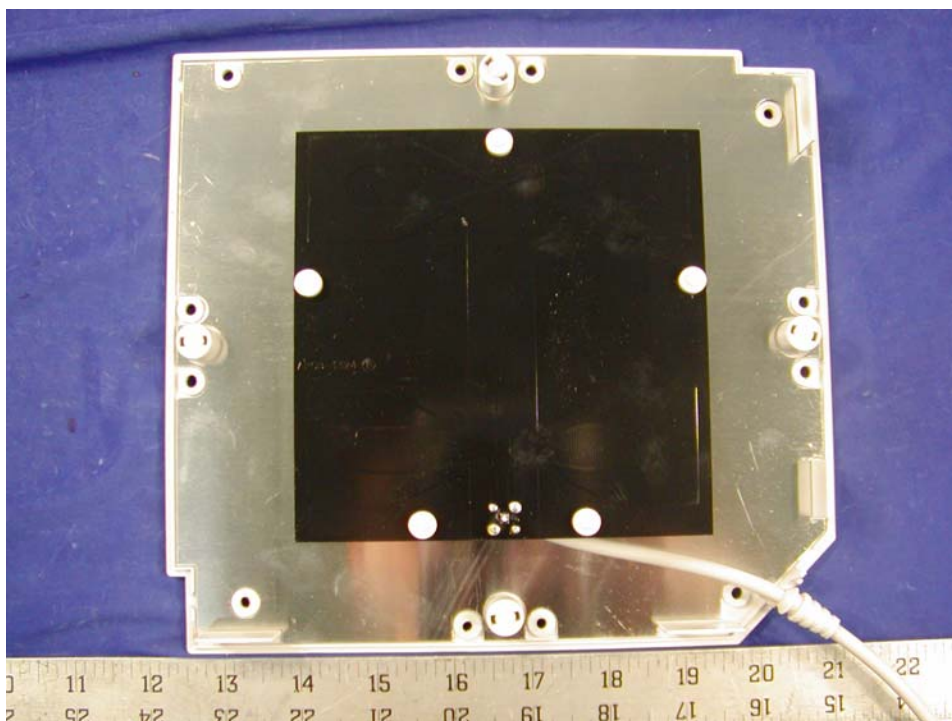
13dBi MP24013 Antenna - Cover Off View
