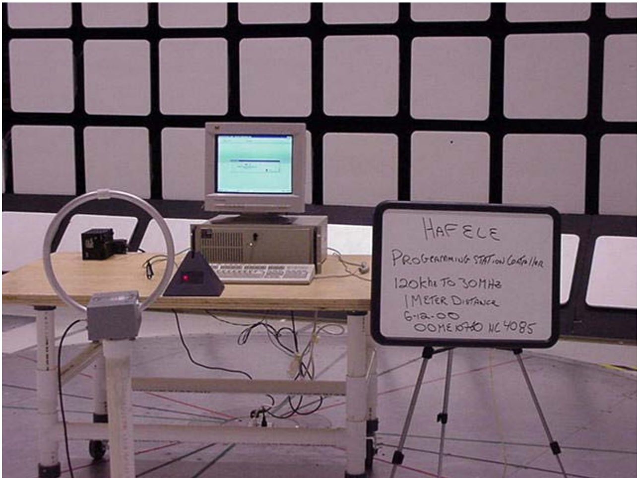
Radiated Emission Test .1 – 30MHz
