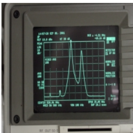
Adjacent channel spurious Output @ 1100 watts peak
