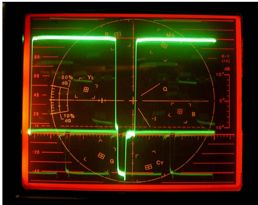
Fig. 2 Two Lines of video showing proper Modulation depth
