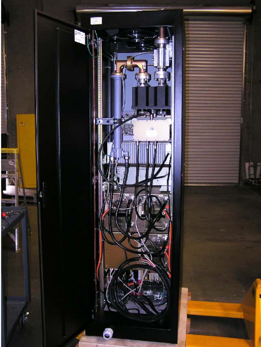
INTERNAL CONSTRUCTION—REAR DOOR OPEN
