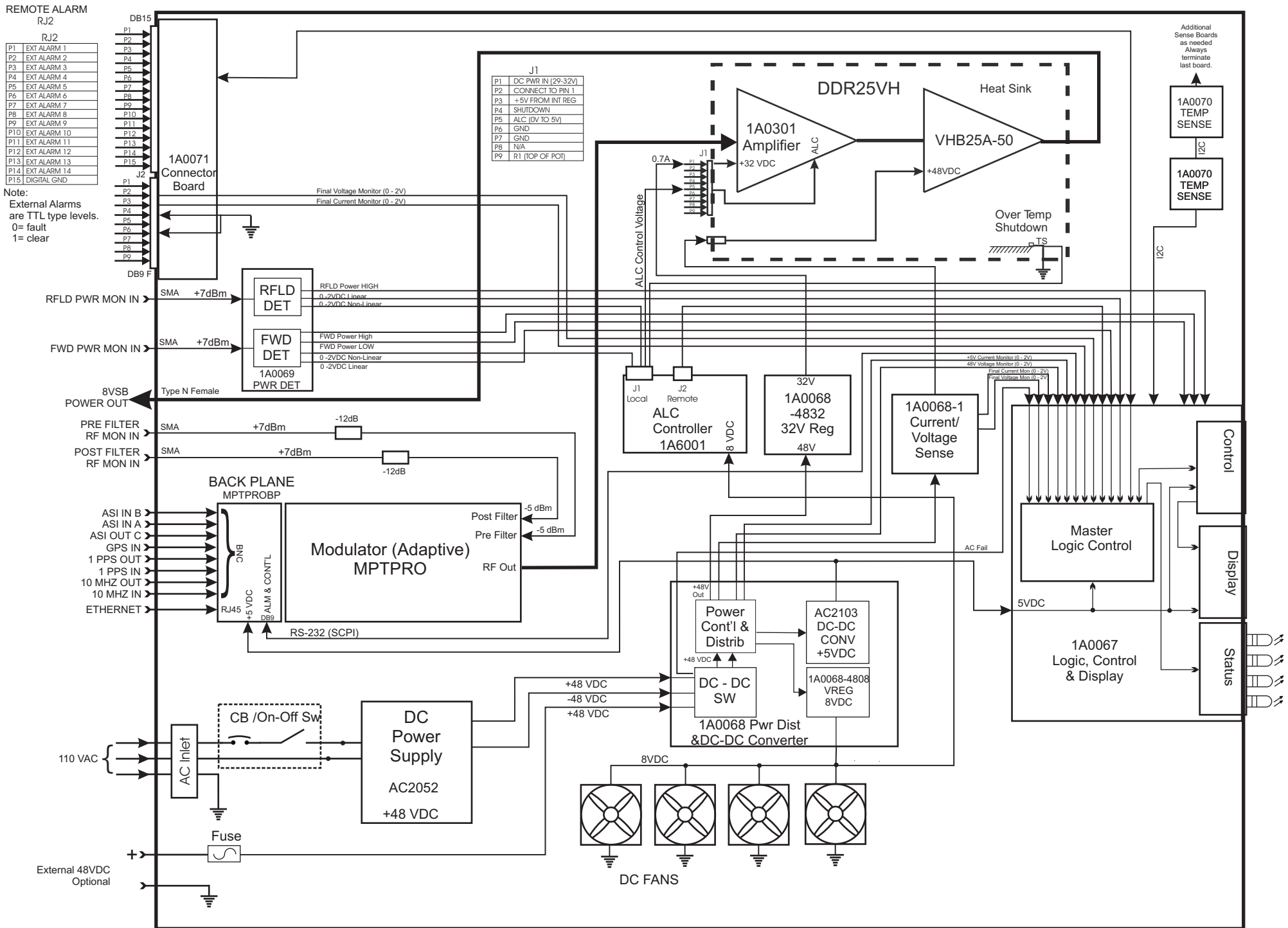
DXDPRO-10VH DIGITAL MODULATOR (Used in DTXPRO-10VH & DTXPRO-400 AND HIGHER TRANSMITTERS)
