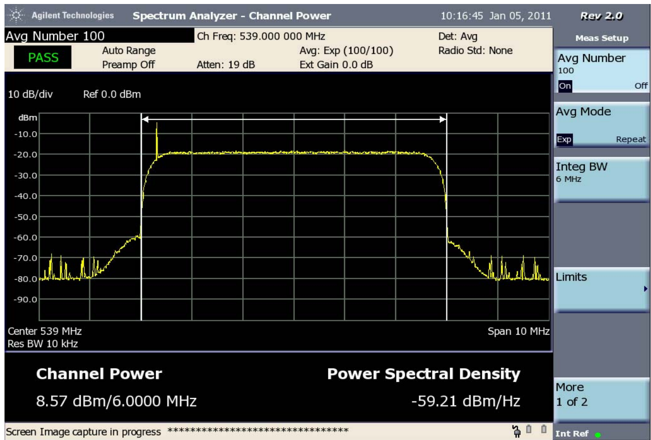
Screenshot 1 - Channel power measured at 539 MHz
