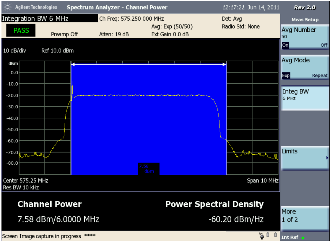
Screenshot 1 - Channel power measured at 575.25 MHz
