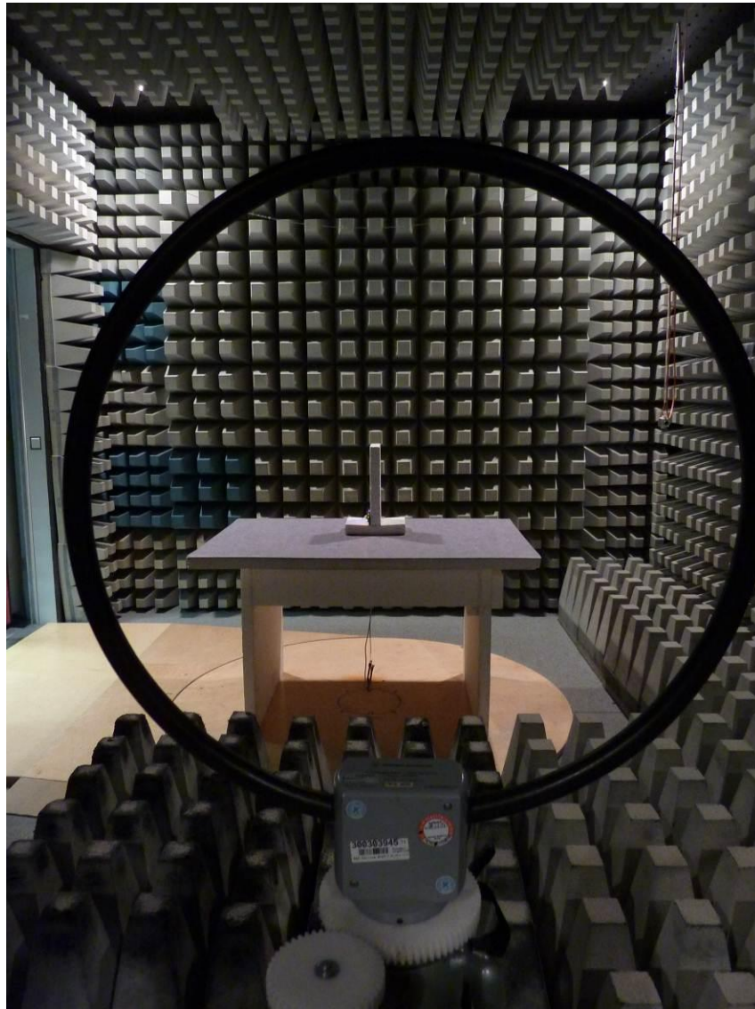
145298_17.jpg: Test setup - Radiated emission (fully anechoic chamber)
