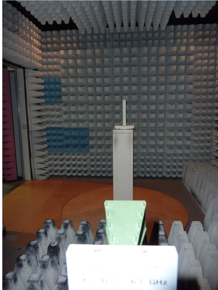
145298_15.jpg: Test setup - Radiated emission (fully anechoic chamber)
