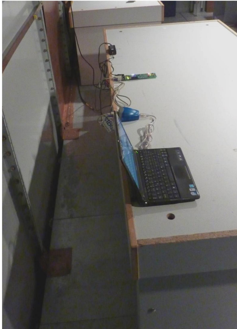
145298_18.jpg: Test setup – conducted emissions on power supply lines
