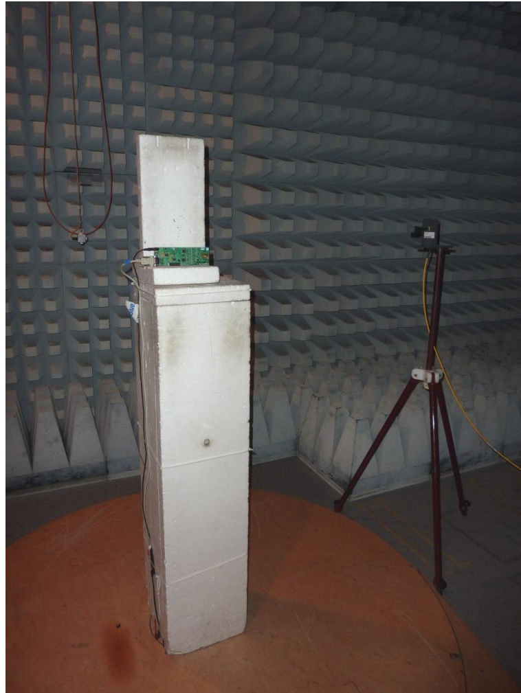
145298_16.jpg: Test setup - Radiated emission (fully anechoic chamber)
