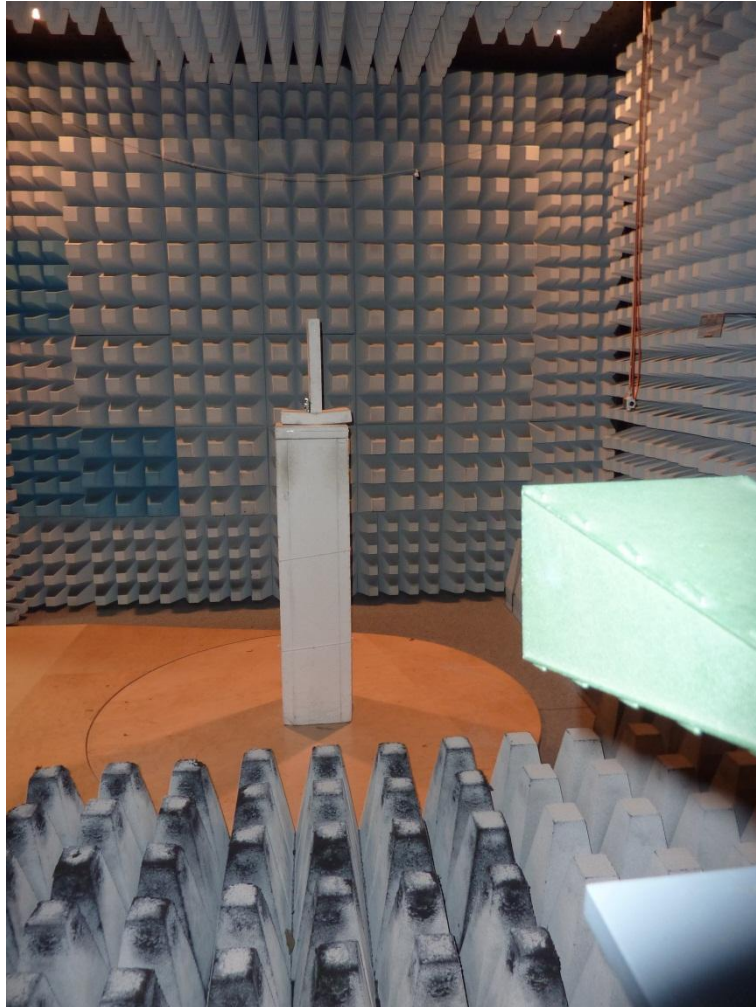
145298_14.jpg: Test setup - Radiated emission (fully anechoic chamber)
