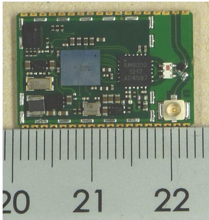
145298_09.JPG: EUT - top view, shielding removed
