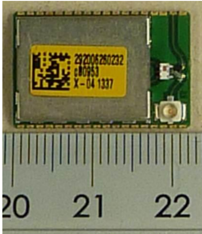
145298_08.JPG: EUT - top view, with shielding
