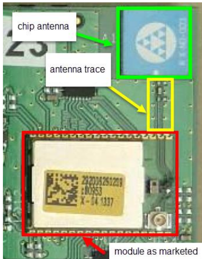
145298_35.jpg: Reference Design with EUT– Detail Top View
