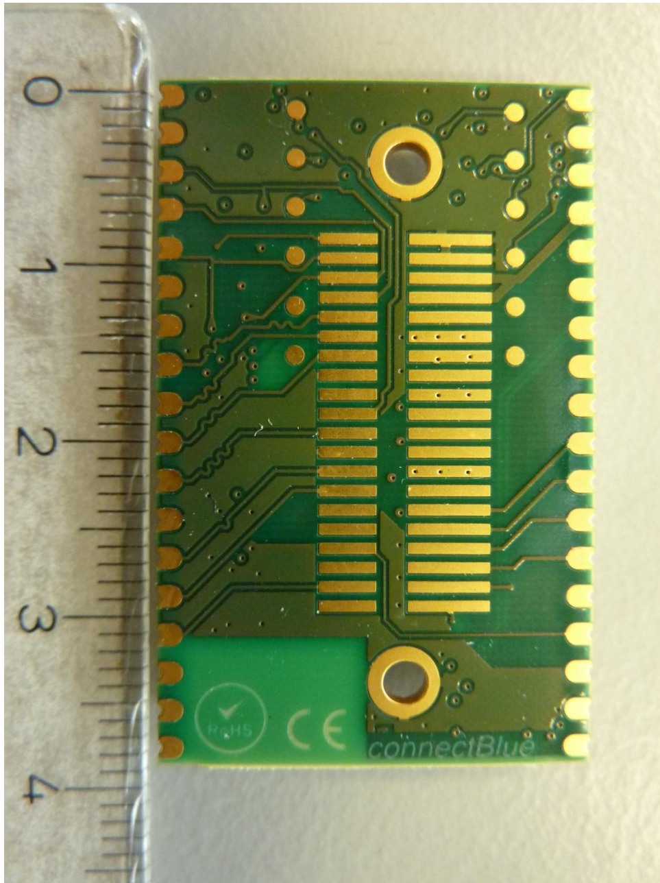
136117_DFS4.JPG: ODIN-W160 (cB-driver), soldered on cB-0957, bottom view
