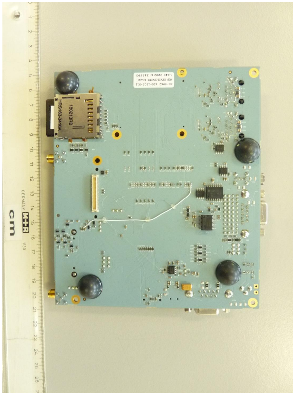
136117_DFS8.JPG: cB-0962 WGP development board, bottom view
