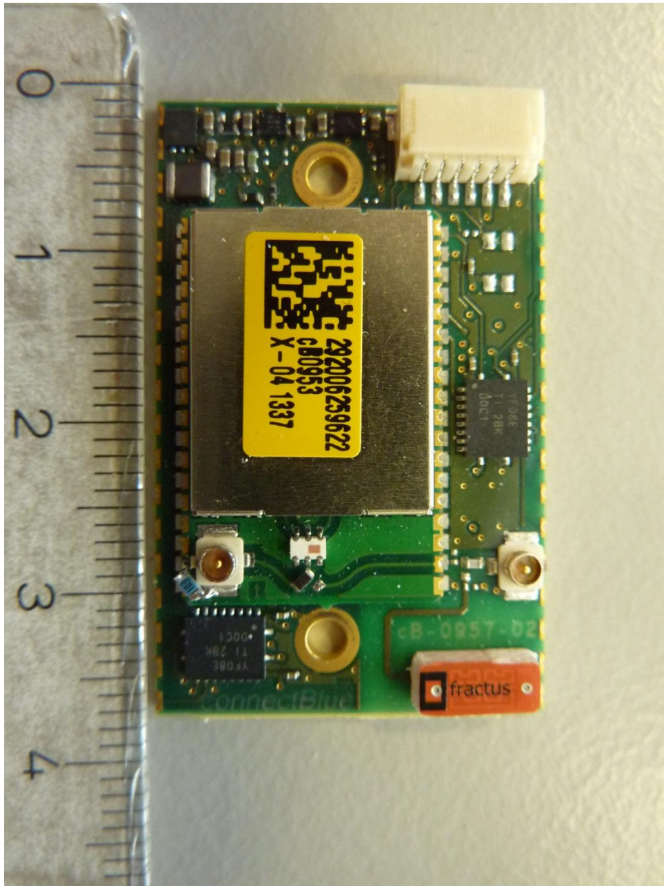
136117_DFS3.JPG: ODIN-W160 (cB-driver), soldered on cB-0957, top view
