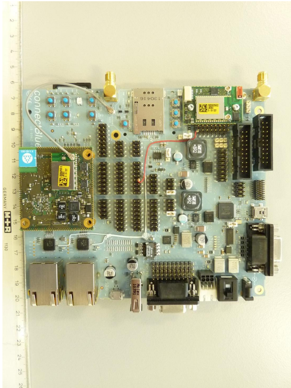
136117_DFS7.JPG: cB-0962 WGP development board, top view
