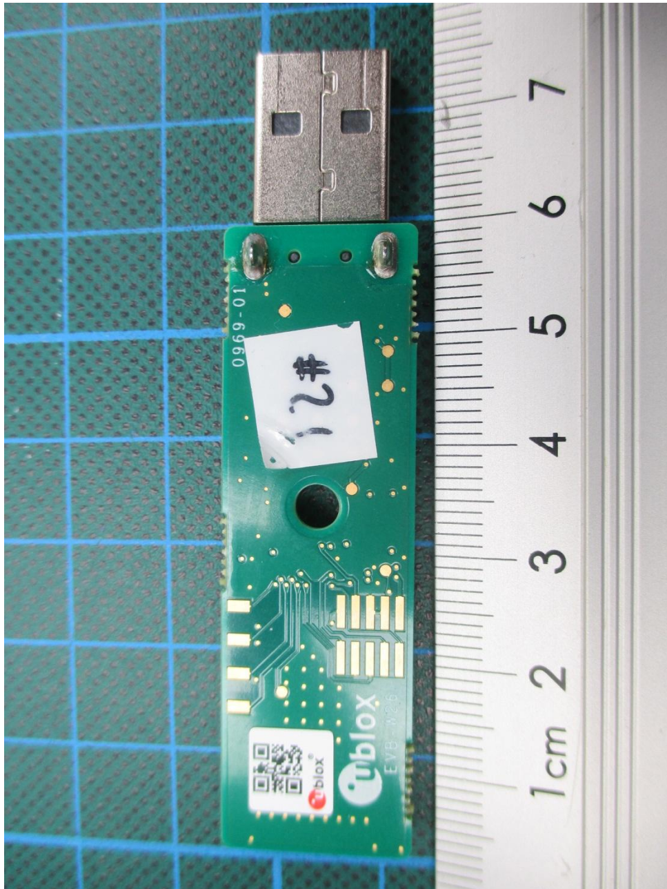
151496_DFS5.JPG: Carrier board, bottom view
