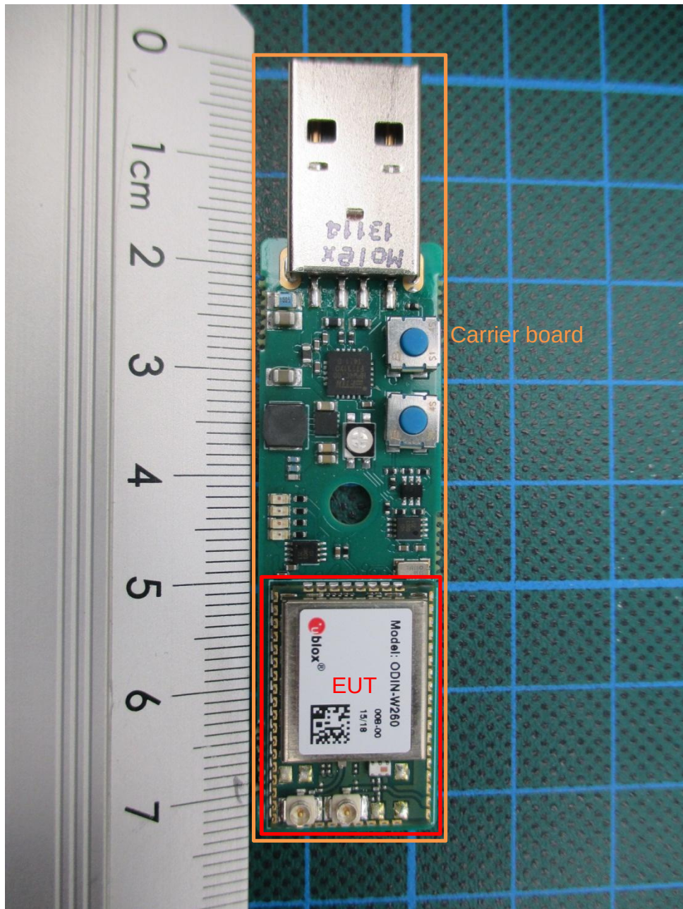
151496_DFS4.JPG: ODIN-W260 mounted on carrier board, top view
