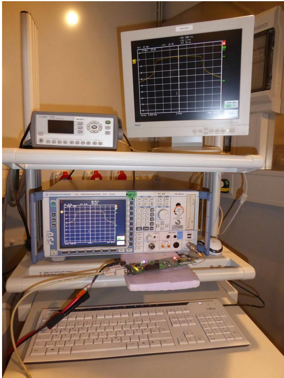
160912_1.jpg: Test setup - conducted tests
