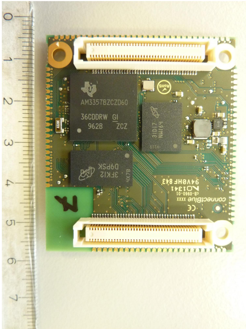
136117_DFS6.JPG: ODIN-W160 (TI-driver), soldered on cB-0960, bottom view
