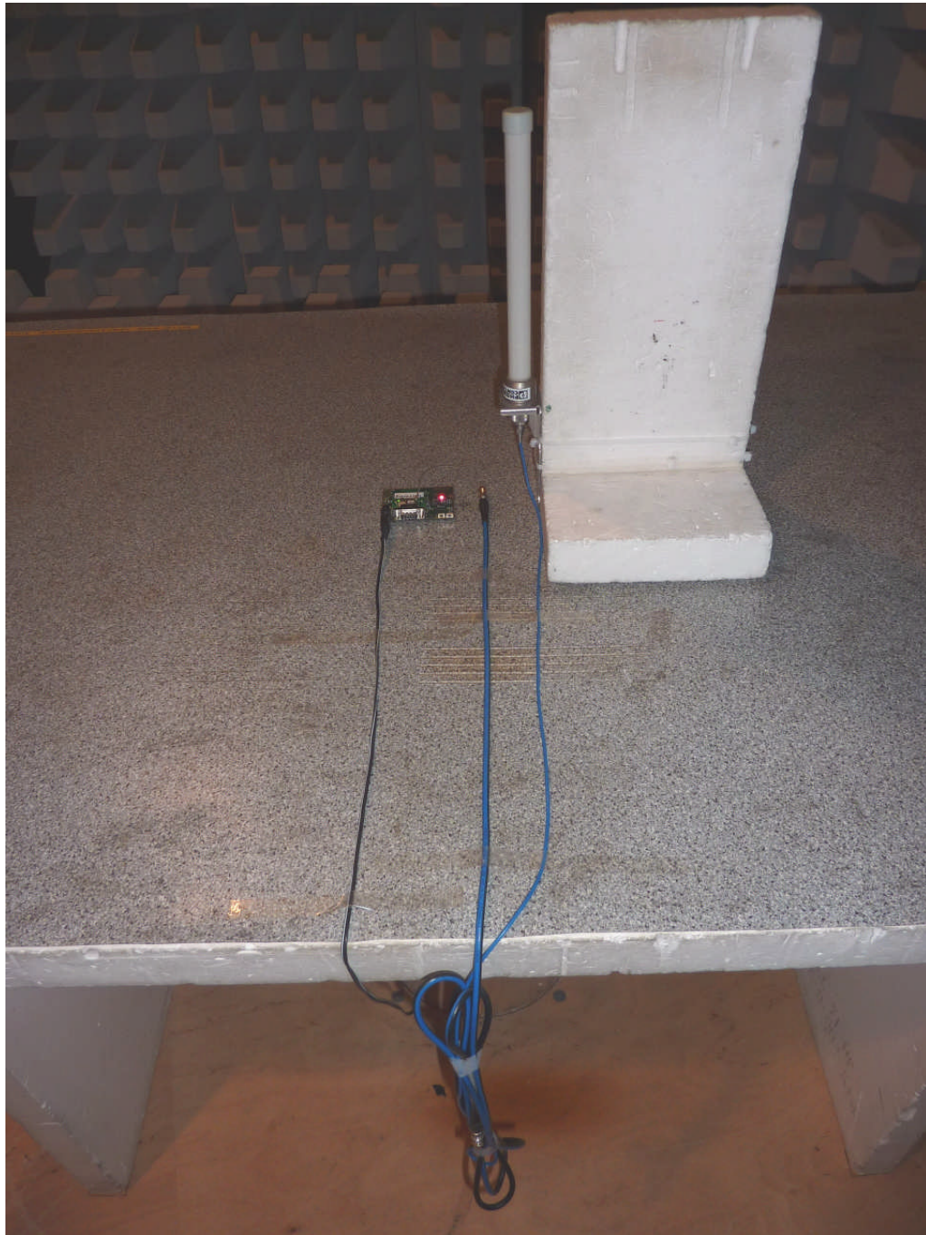
120262_8.JPG: cB-0950 with external monopole antenna, test set-up fully anechoic chamber (pos. 1)
