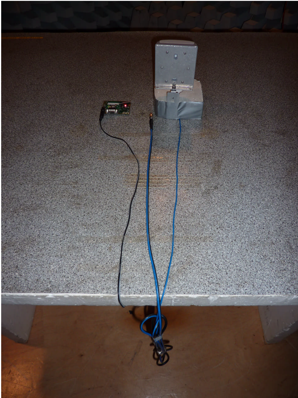
120262_6.JPG: cB-0950 with external patch antenna, test set-up fully anechoic chamber (pos. 1)
