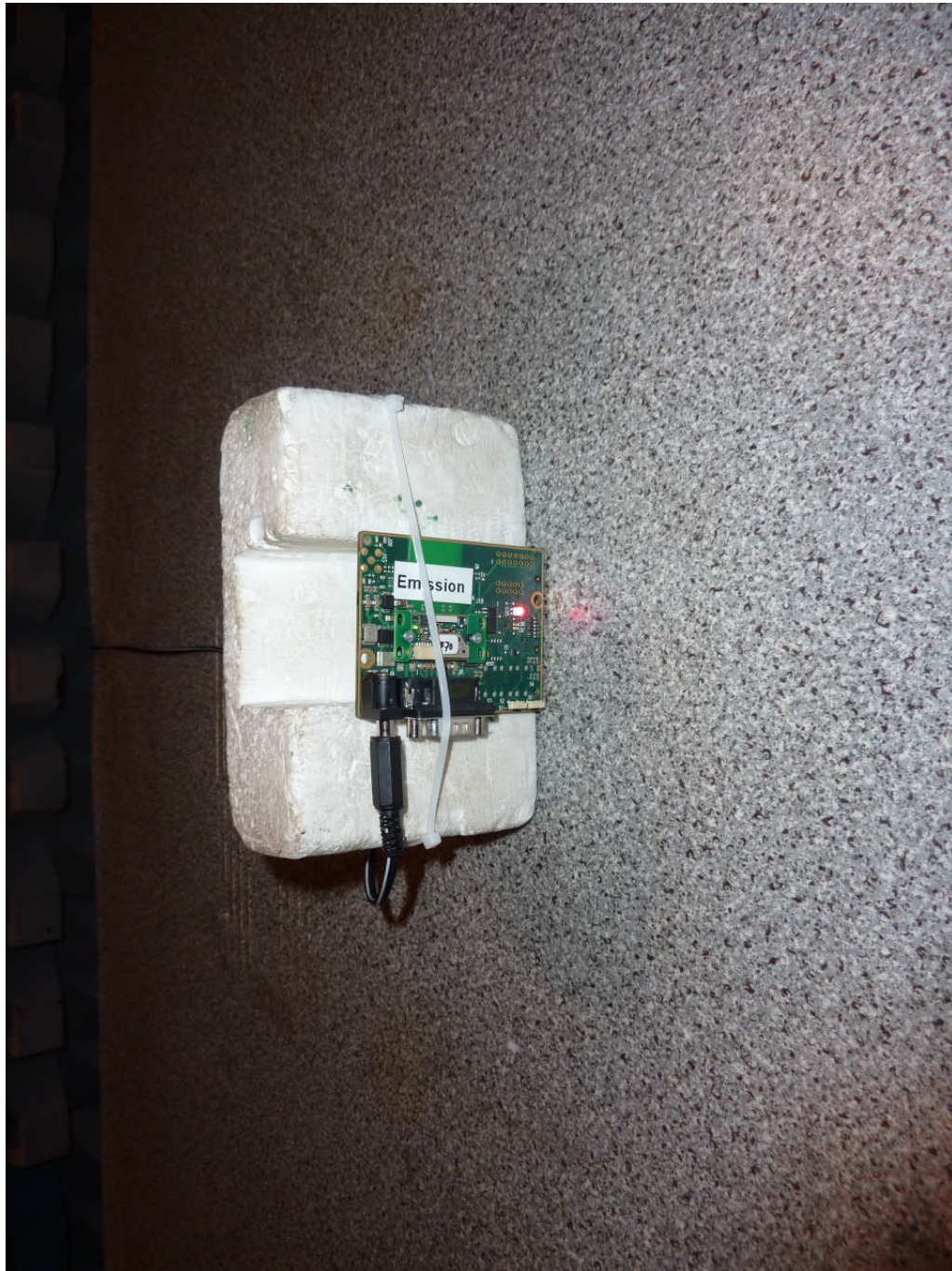
120262_4.JPG: cB-0950 with internal antenna, test set-up fully anechoic chamber (pos. 1)
