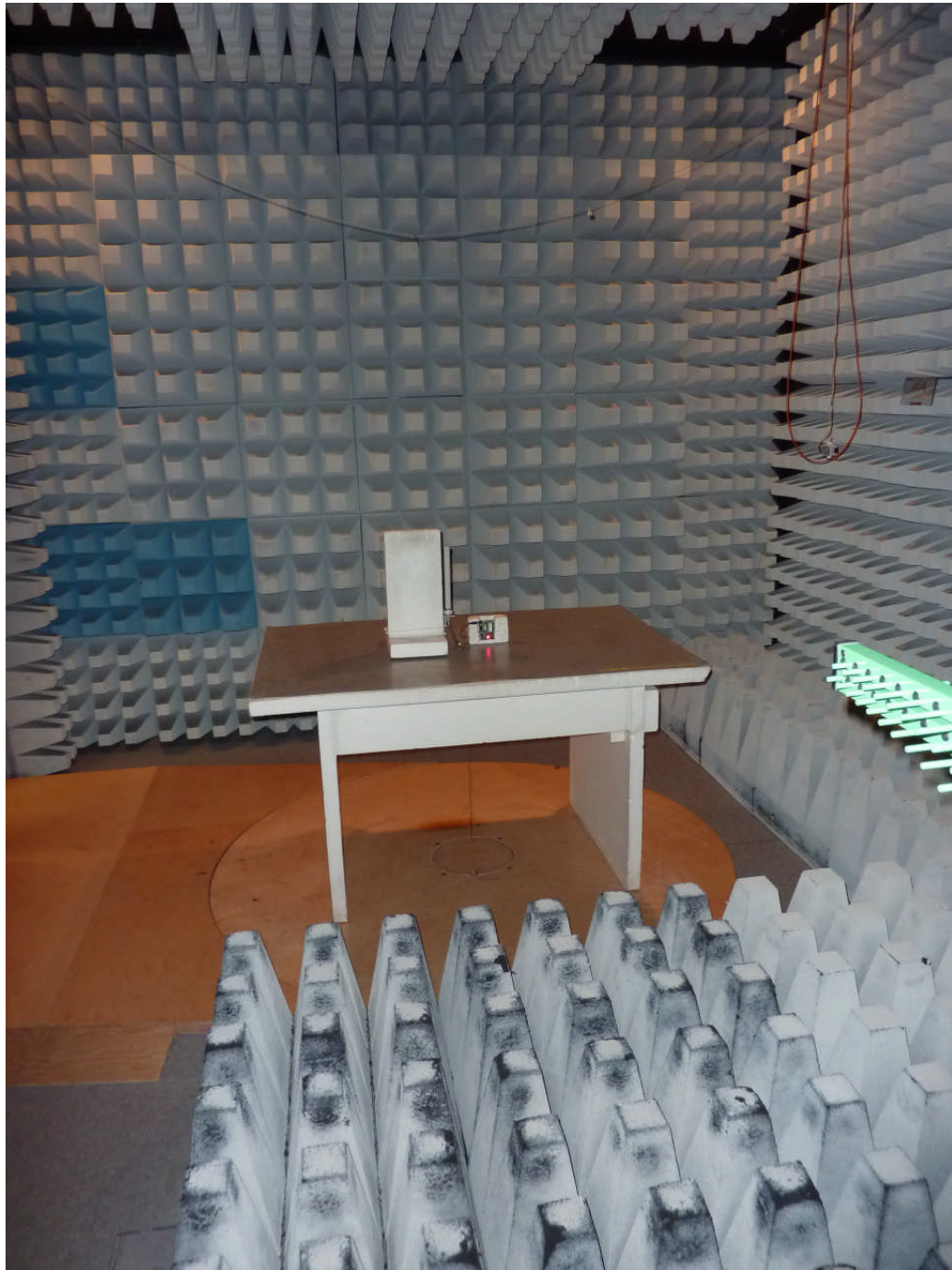
120262_13.JPG: cB-0950 with external monopole antenna (pos. 2), test set-up fully anechoic chamber
