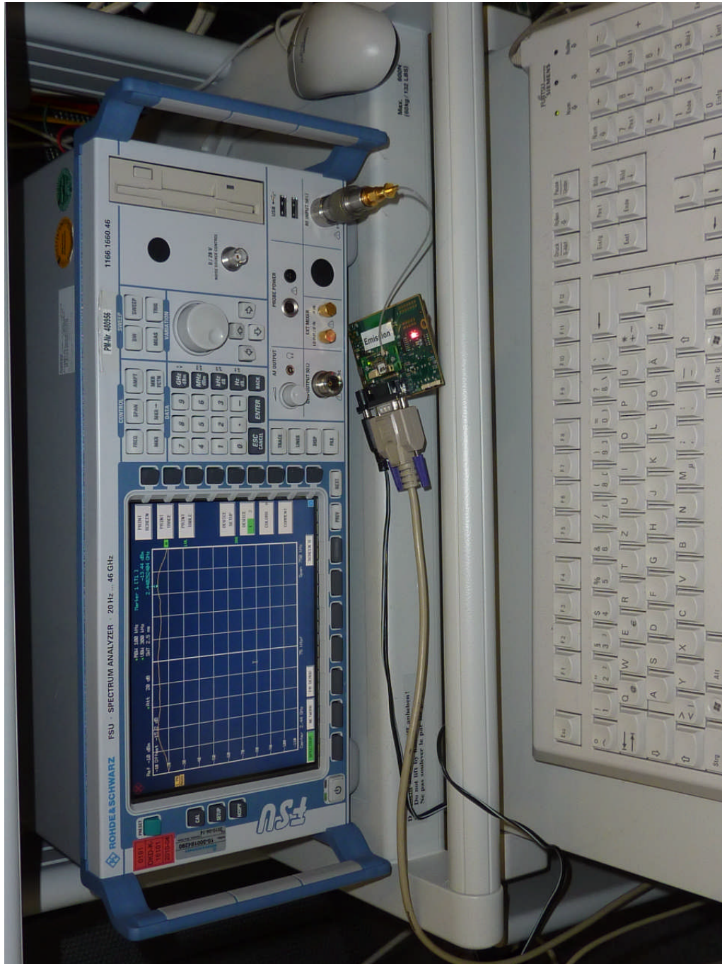
120262_34.JPG: cB-0950, test set-up conducted measurements
