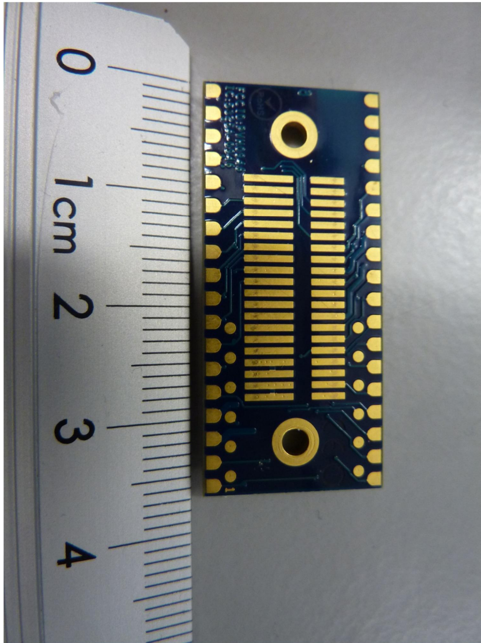
124266_11.JPG: cB-0946, PCB bottom view
