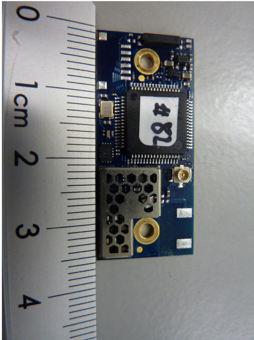
124266_12.JPG: cB-0946 with antenna connector, PCB top view
