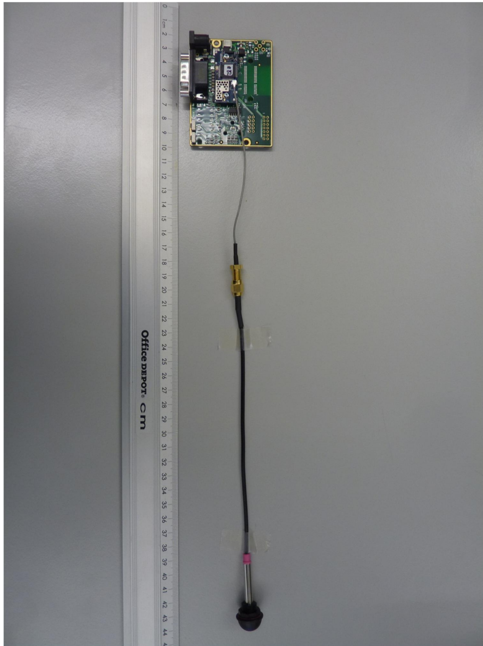
124266_7.JPG: cB-0946 mounted on cB-0903-03 with connected ANT-2.4-WRT-xxx
