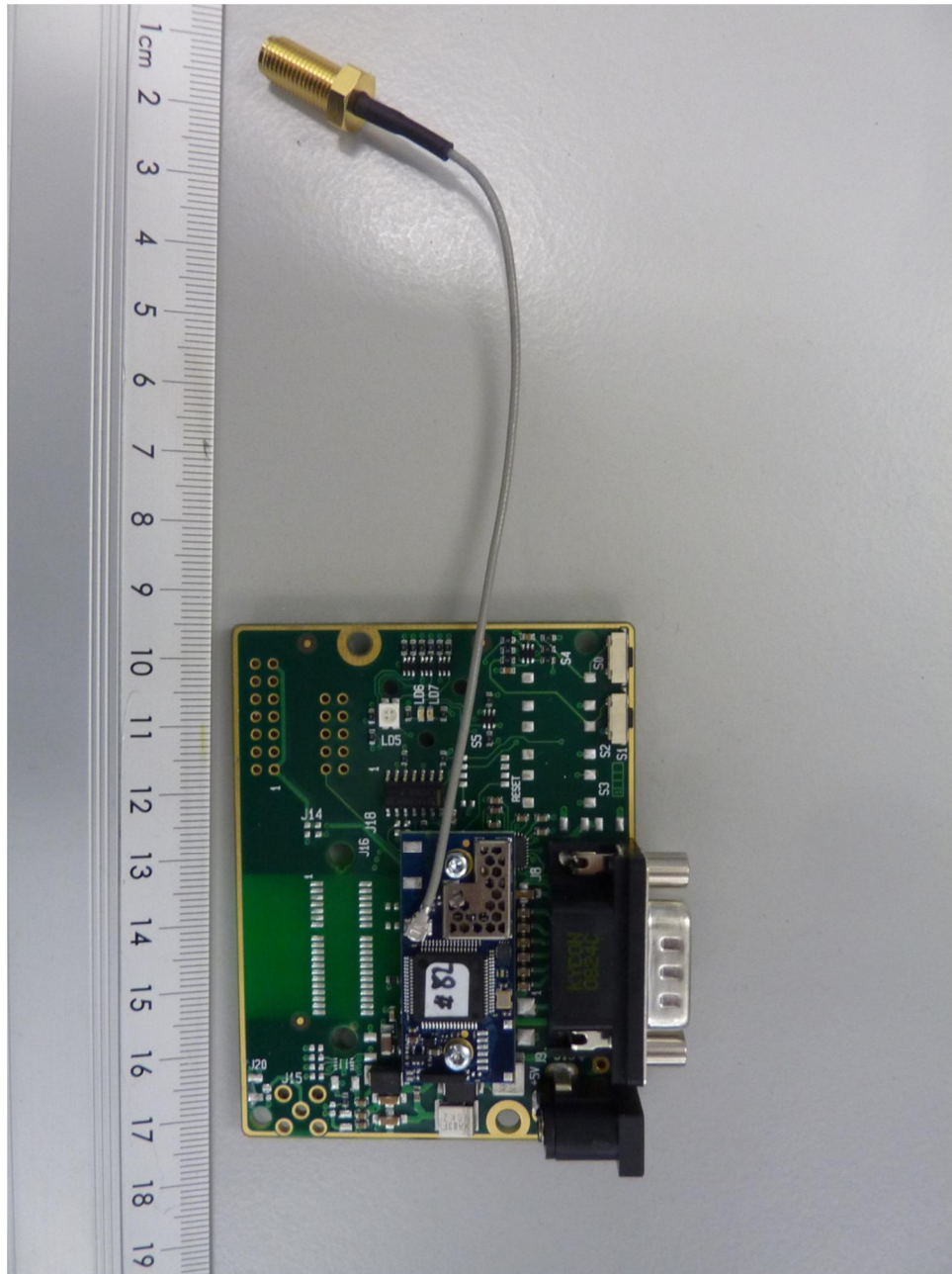
124266_10.JPG: cB-0946 mounted on the cB-0903-03 (carrier board)
