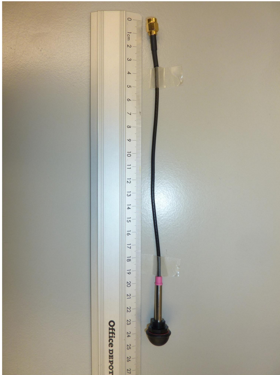
124266_8.JPG: ANT-2.4-WRT-xxx
