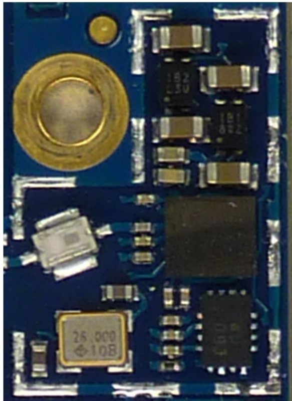
124266_13.JPG: cB-0946, Shielding removed, top wiew
