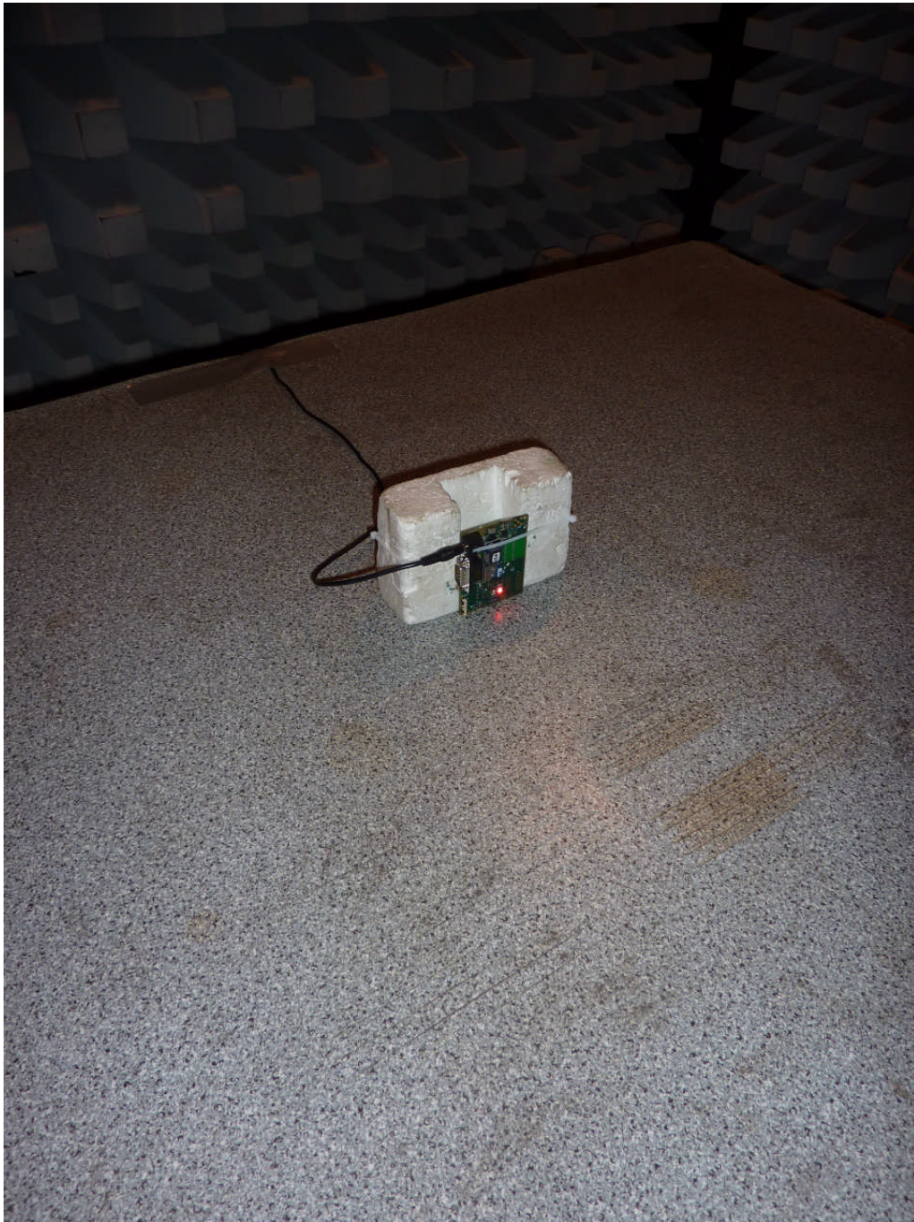
111592_42.JPG: cB-0946 with internal antenna, test setup fully anechoic chamber (pos. 2)
