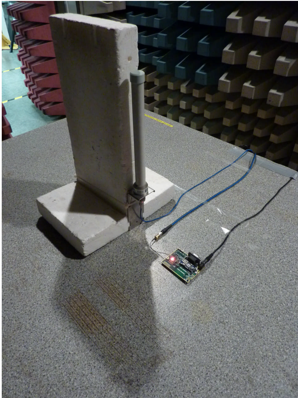
111592_46.JPG: cB-0946 with external monopole antenna, test setup fully anechoic chamber (pos. 1)
