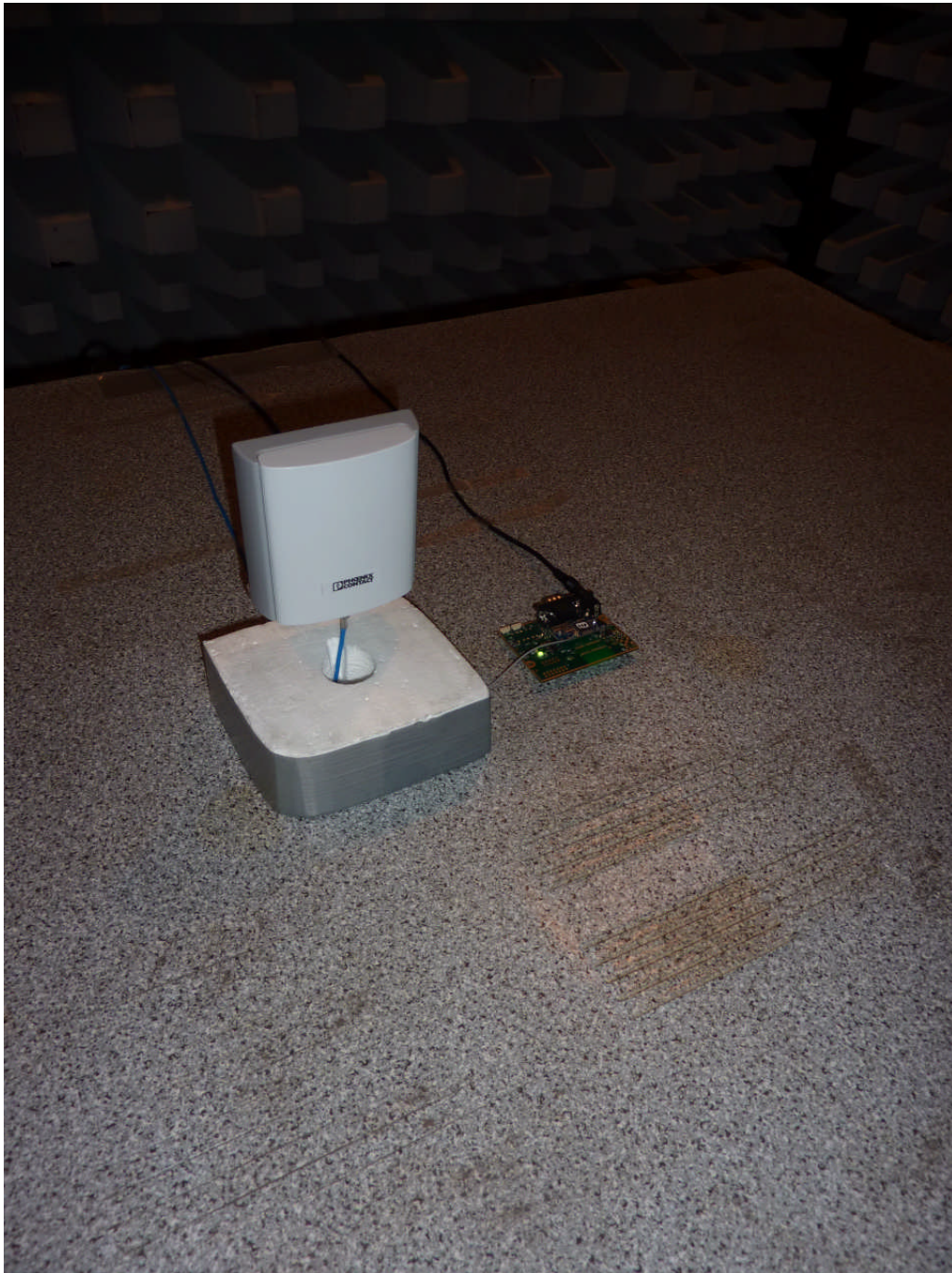
111592_43.JPG: cB-0946 with external patch antenna, test setup fully anechoic chamber (pos. 1)
