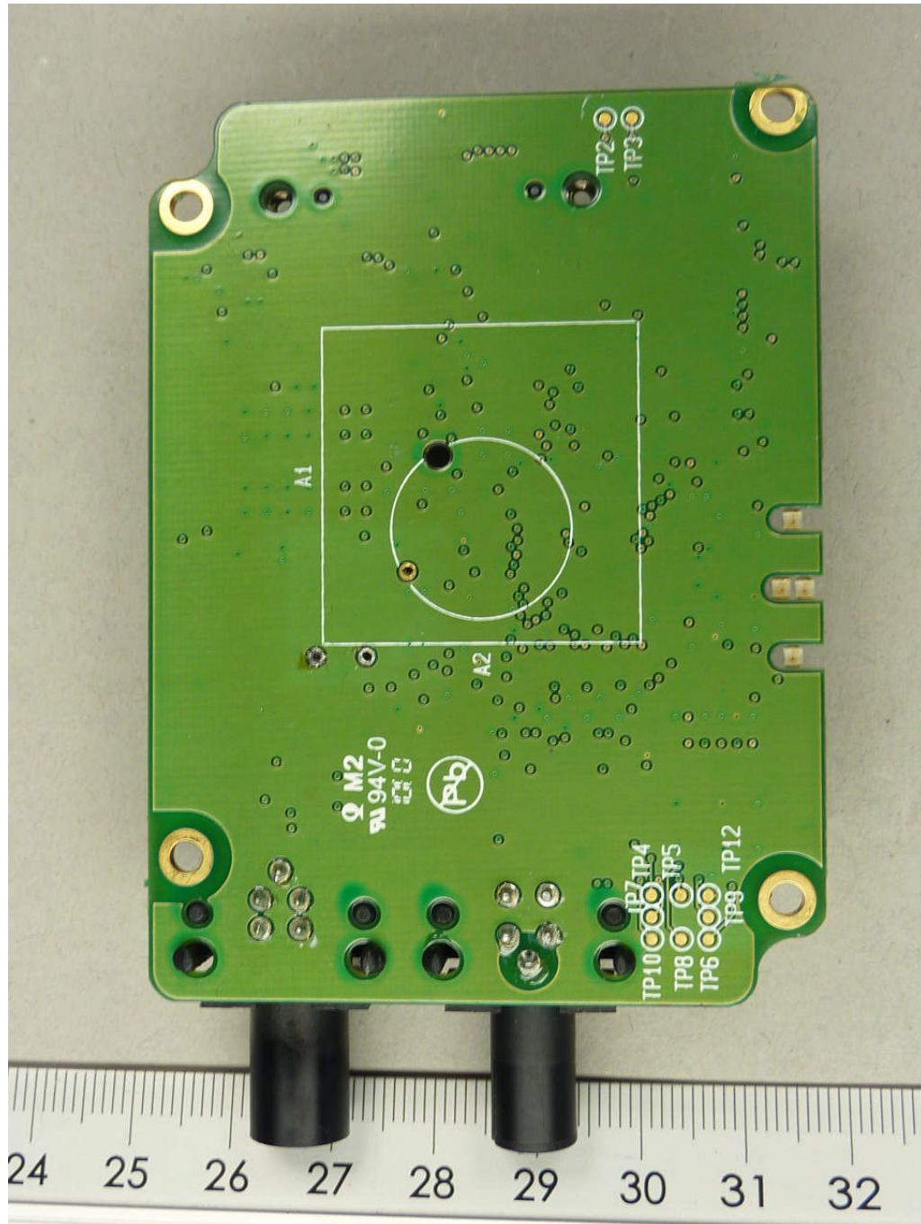
111592_m.JPG: cB-0924-02, bottom view, antenna removed
