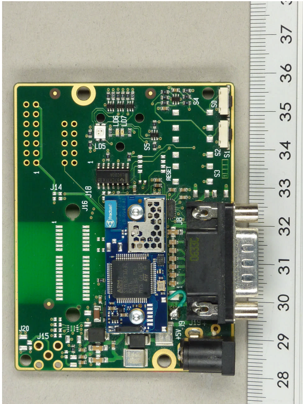
111592_b.JPG: cB-0946 mounted on the cB-0903-03 (carrier board)
