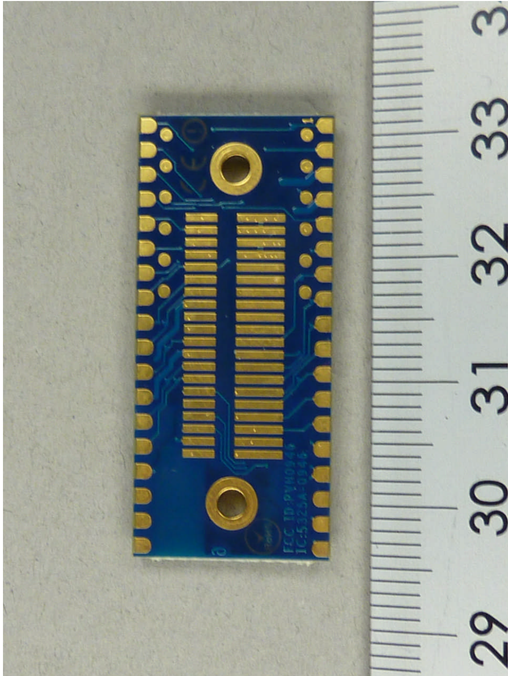
111592_f.JPG: cB-0946, PCB, bottom view
