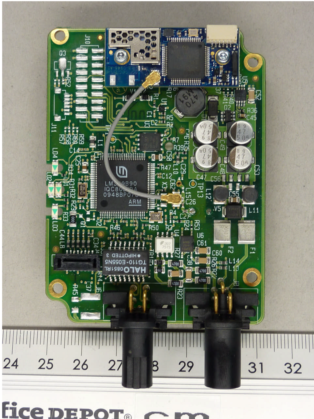
111592_j.JPG: cB-0946 mounted on the cB-0924-02 (EPA)
