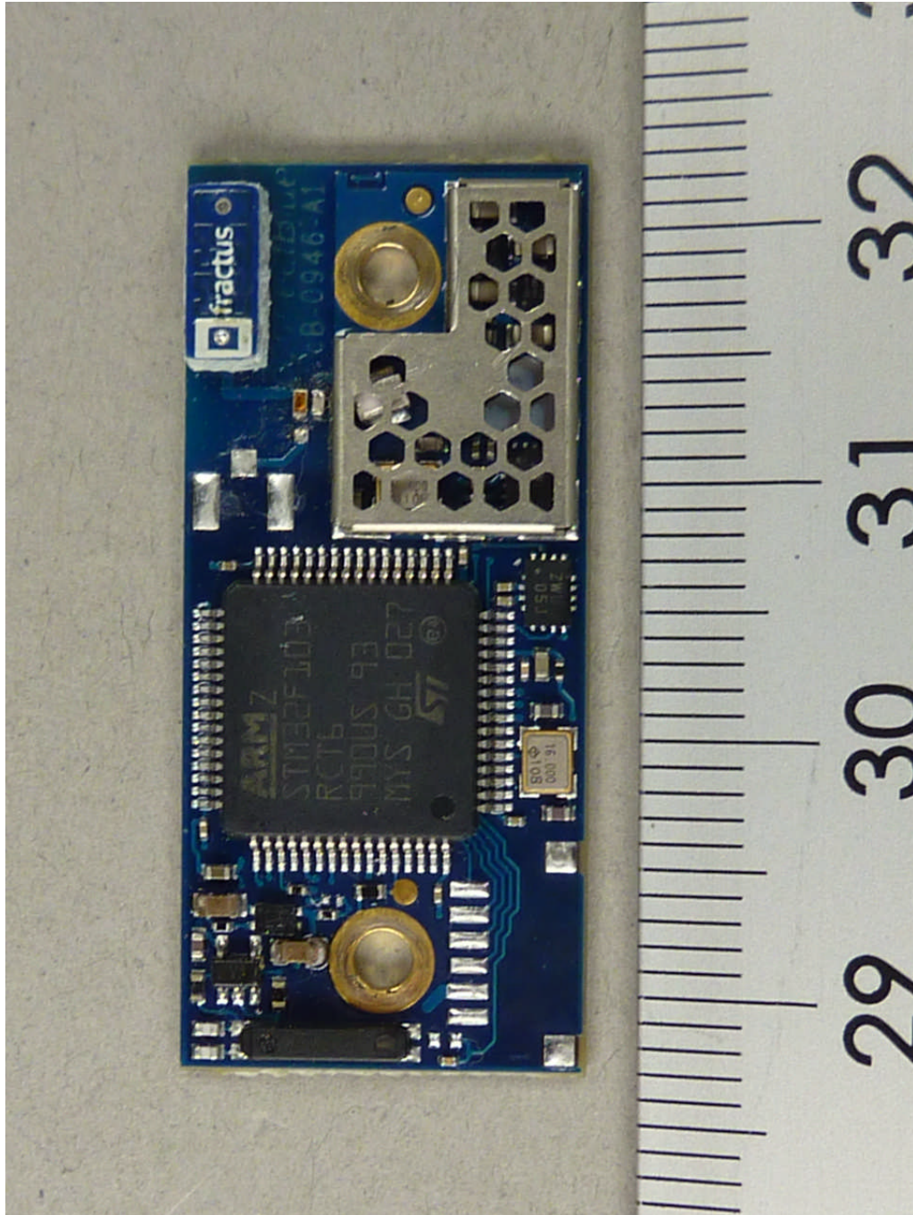
111592_i.JPG: cB-0946 with internal antenna, PCB, top view
