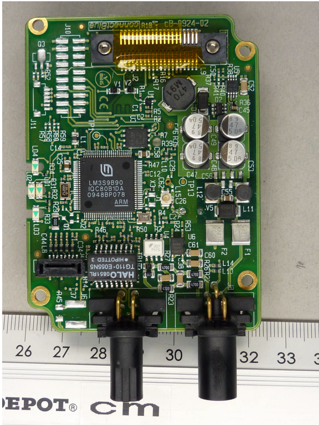
111592_I.JPG: cB-0924-02, top view
