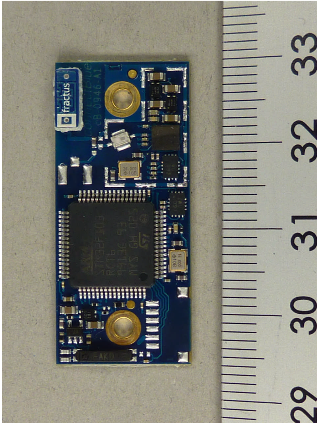
111592_h.JPG: cB-0946 with internal antenna, PCB, top view, shielding removed
