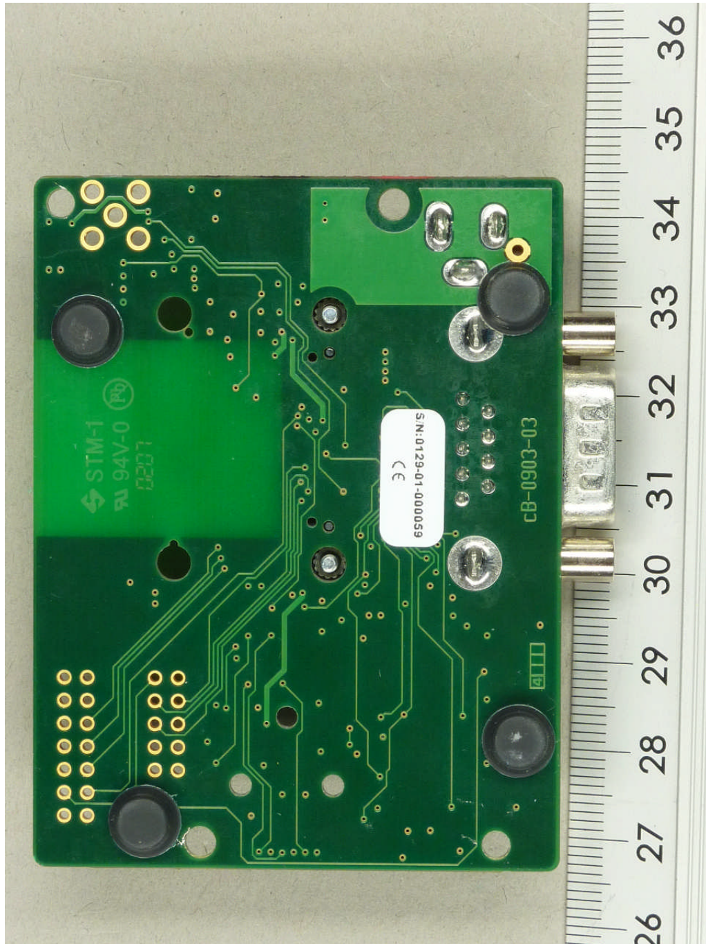
111592_c.JPG: cB-0903, PCB, bottom view
