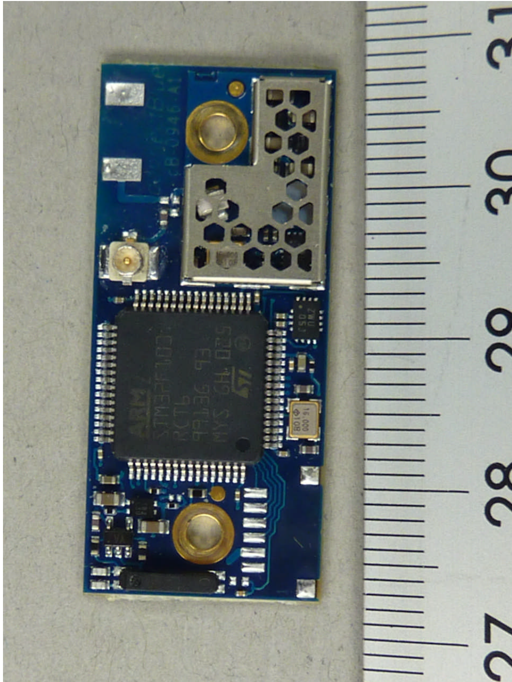
111592_g.JPG: cB-0946 with antenna connector, PCB, top view
