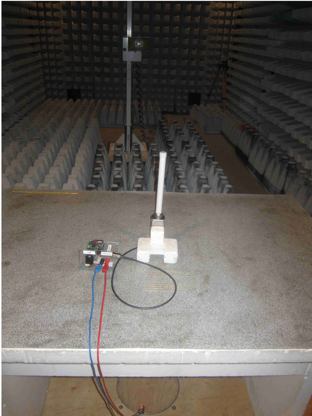
120198_17: Test setup - Radiated emission, Ant 3 (fully anechoic chamber)
