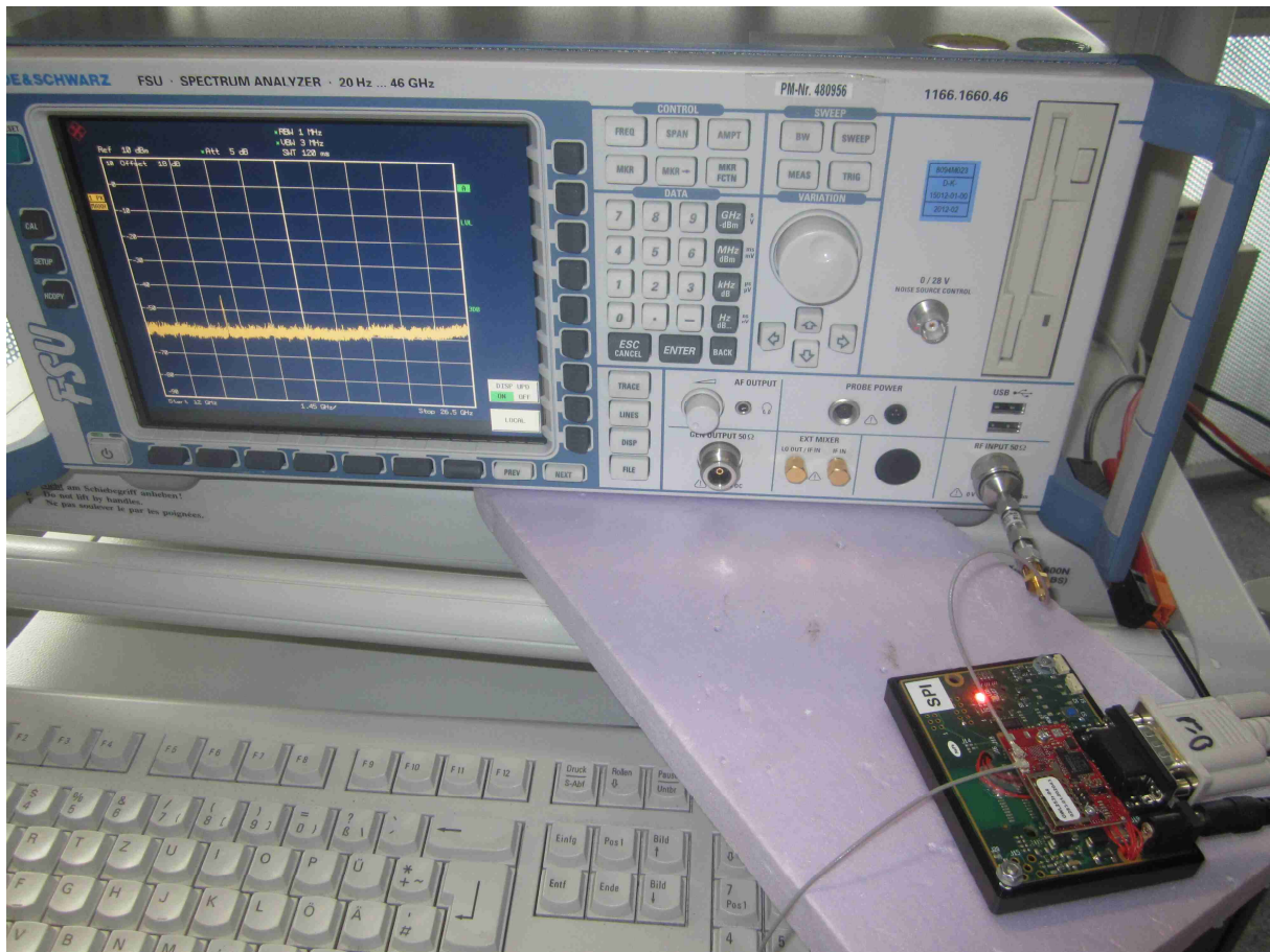
120198_06: Test setup – conducted emissions
