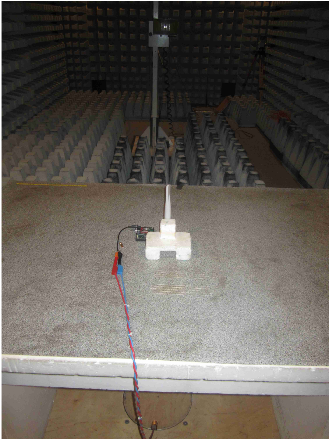
120198_05: Test setup - Radiated emission, Ant 4 (fully anechoic chamber)
