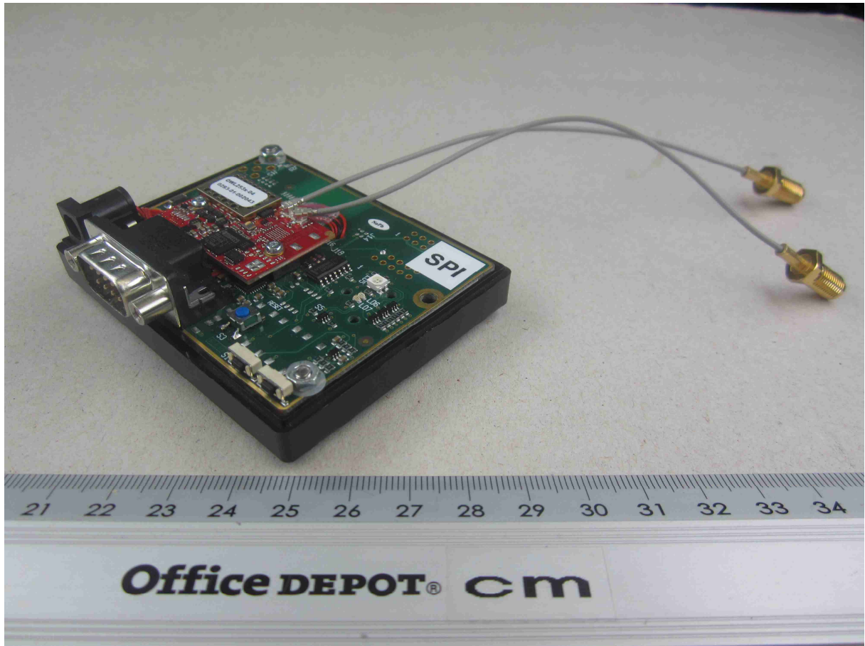
120198_07.JPG: EUT, 3D view 1
