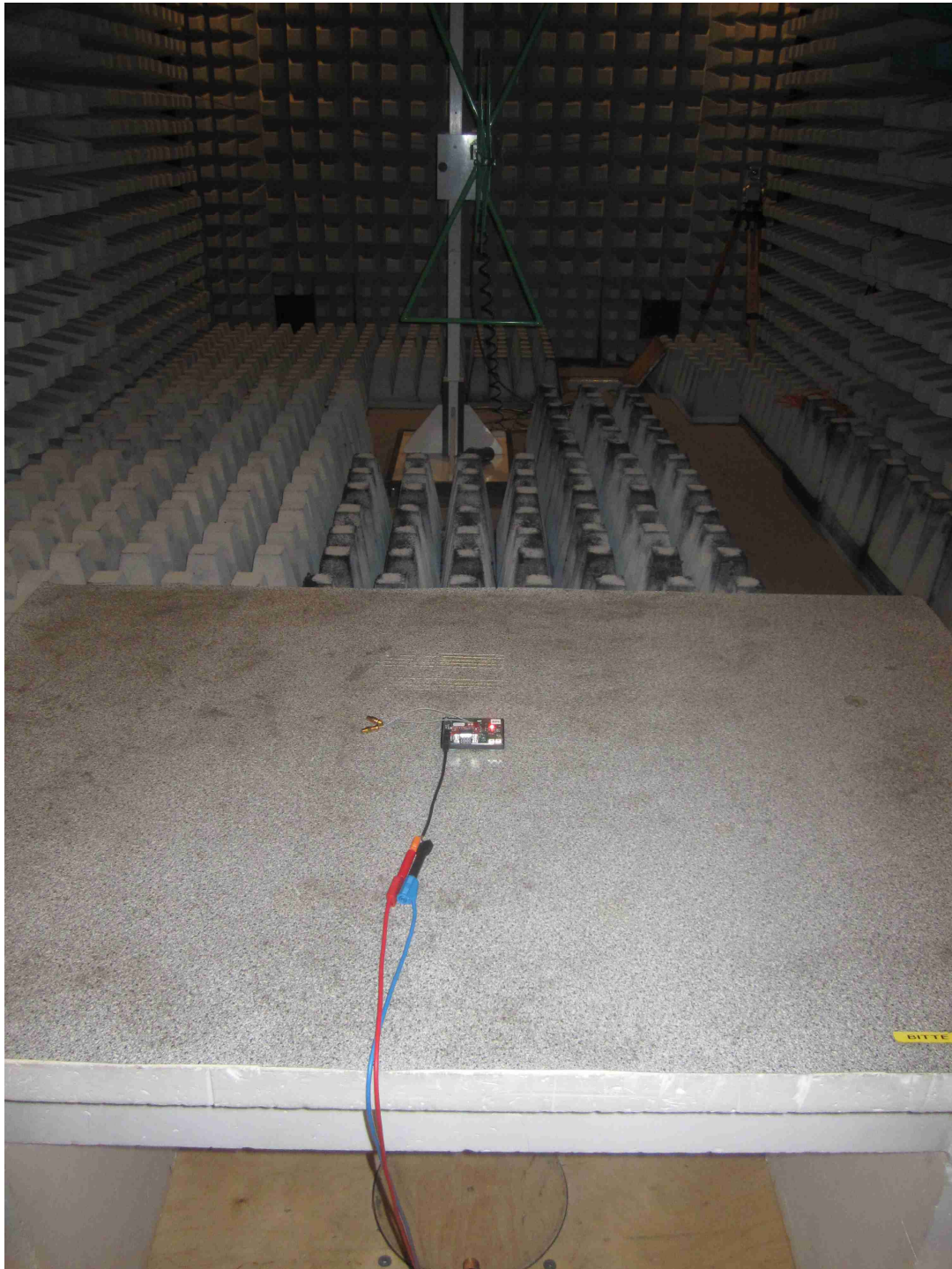
120198_01: Test setup - Radiated emission, Antennas terminated (fully anechoic chamber)
