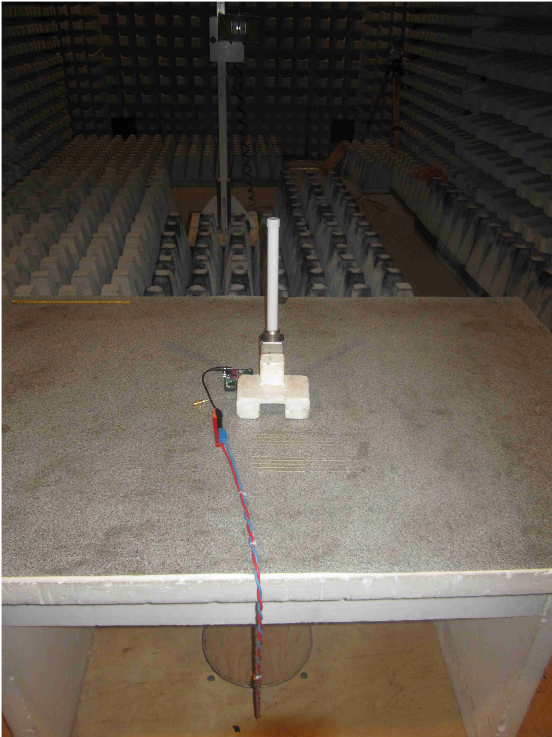
120198_03: Test setup - Radiated emission, Ant 1 (fully anechoic chamber)
