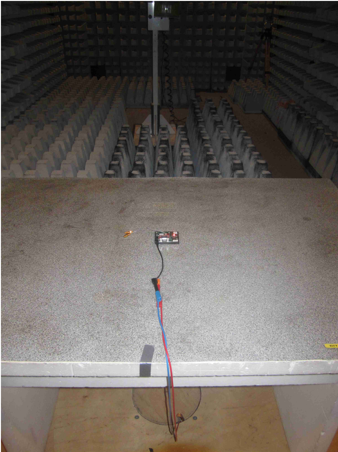
120198_02: Test setup - Radiated emission, Antennas terminated (fully anechoic chamber)
