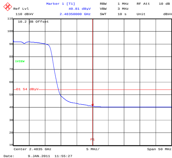
BandEdge_802_11G_24MBS_TopChannelAVG
