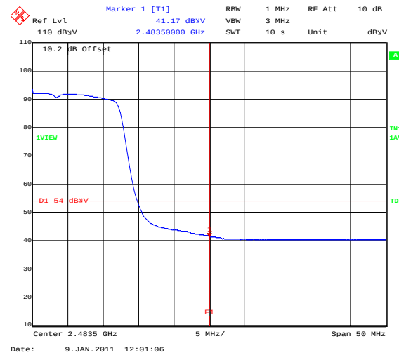
BandEdge_802_11N_13MBS_TopChannelAVG
