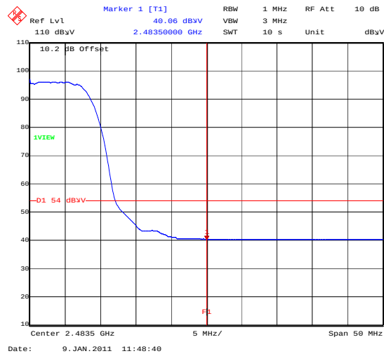
BandEdge_802_11B_5.5MBS_TopChannelAVG
