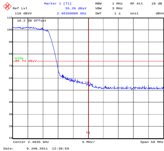
BandEdge_802_11N_26MBS_TopChannel
