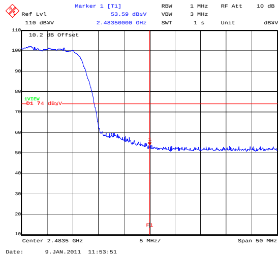
BandEdge_802_11G_18MBS_TopChannel
