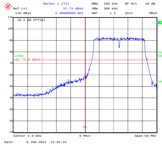
BandEdge_802_11N_26MBS_BotChannel
