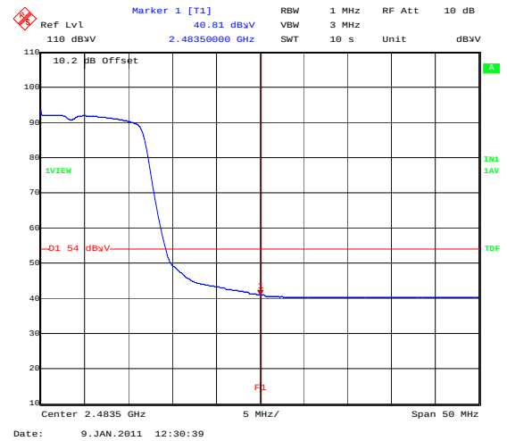
BandEdge_802_11G_54MBS_TopChannelAVG
