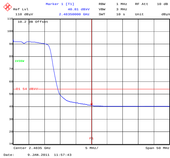
BandEdge_802_11G_48MBS_TopChannelAVG
