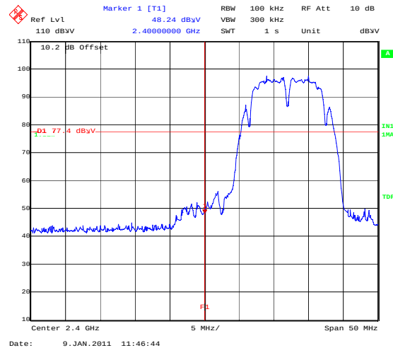
BandEdge_802_11B_2MBS_BotChannel
