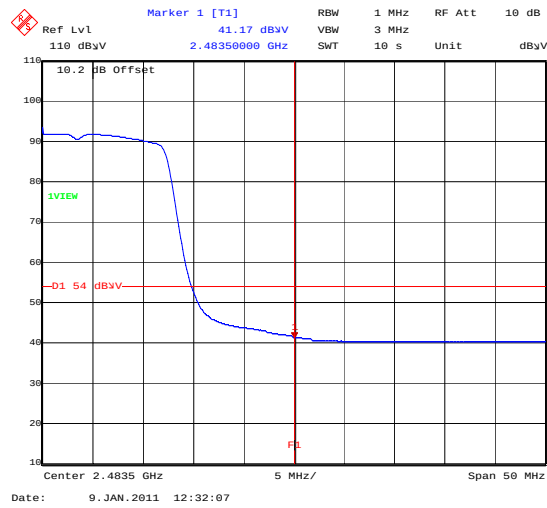
BandEdge_802_11N_58.5MBS_TopChannelAVG
