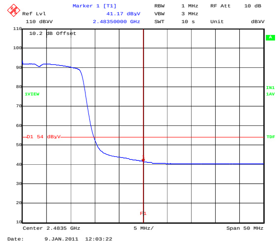
BandEdge_802_11N_26MBS_TopChannelAVG
