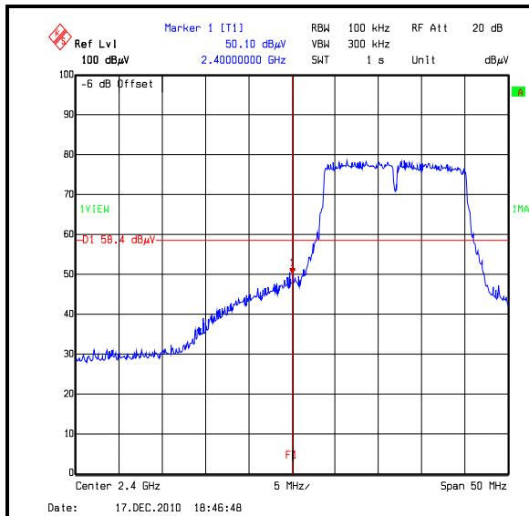
BandEdgeEIRP802_11G_18MBS_BottomChannel
