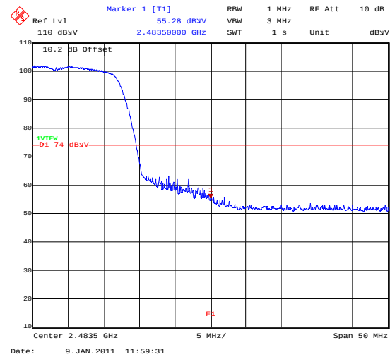
BandEdge_802_11N_6.5MBS_TopChannel
