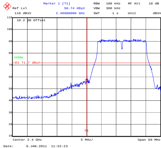
BandEdge_802_11G_12MBS_BotChannel
