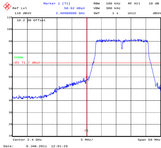
BandEdge_802_11N_19.5MBS_BotChannel
