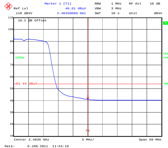
BandEdge_802_11G_18MBS_TopChannelAVG
