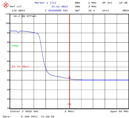
BandEdge_802_11N_6.5MBS_TopChannelAVG
