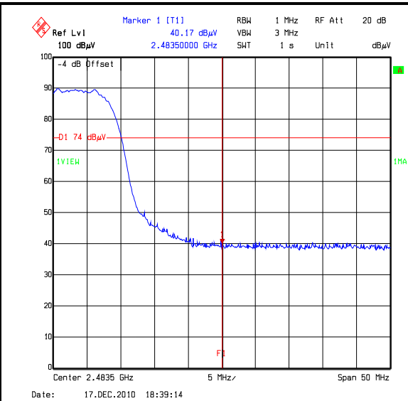
BandEdgeEIRP802_11B_5.5MBS_TopChannel
