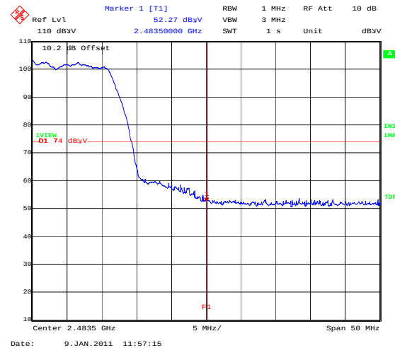
BandEdge_802_11G_48MBS_TopChannel
