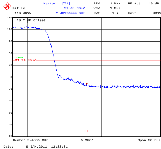
BandEdge_802_11G_54MBS_TopChannel
