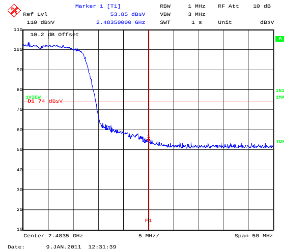
BandEdge_802_11N_58.5MBS_TopChannel
