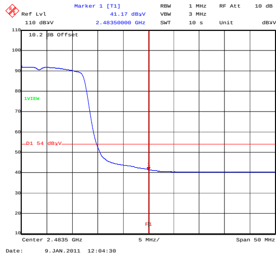
BandEdge_802_11N_39MBS_TopChannelAVG
