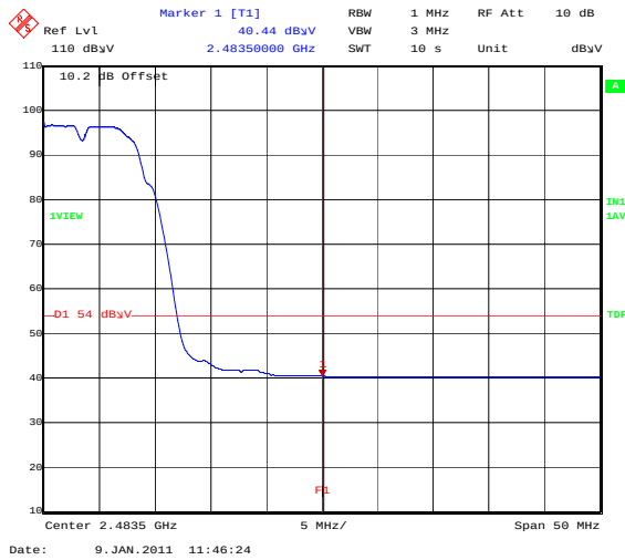
BandEdge_802_11B_1MBS_TopChannelAVG
