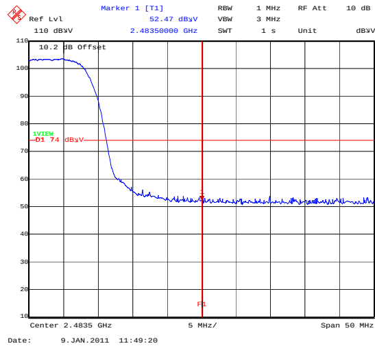
BandEdge_802_11B_11MBS_TopChannel
