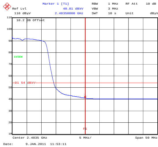
BandEdge_802_11G_12MBS_TopChannelAVG
