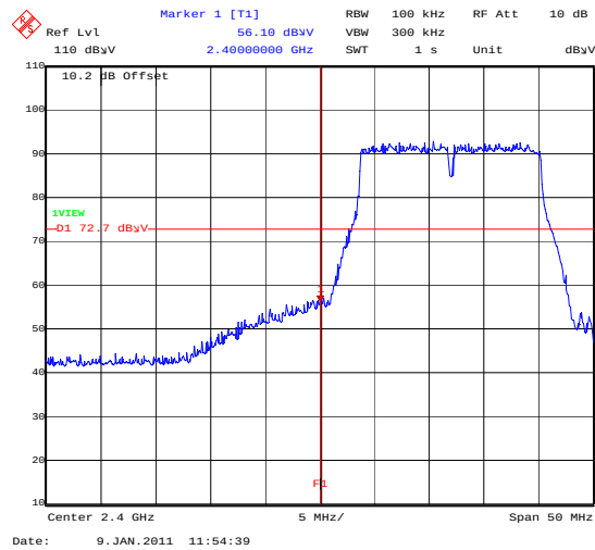
BandEdge_802_11G_24MBS_BotChannel
