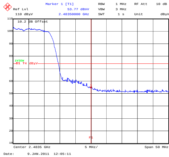
BandEdge_802_11N_52MBS_TopChannel
