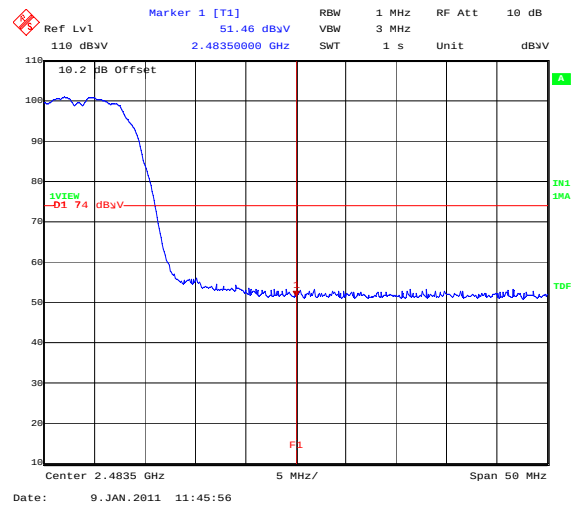
BandEdge_802_11B_1MBS_TopChannel
