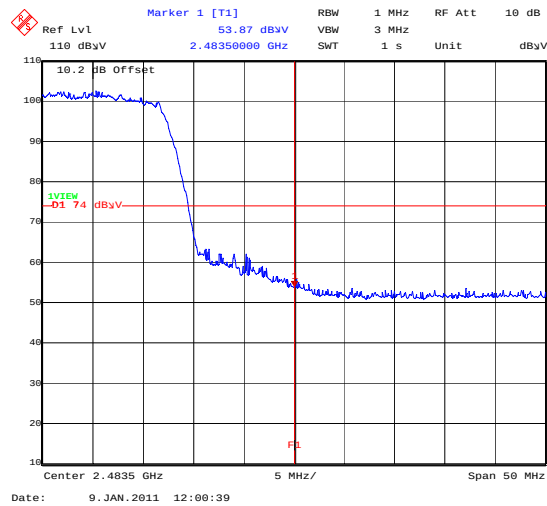
BandEdge_802_11N_13MBS_TopChannel
