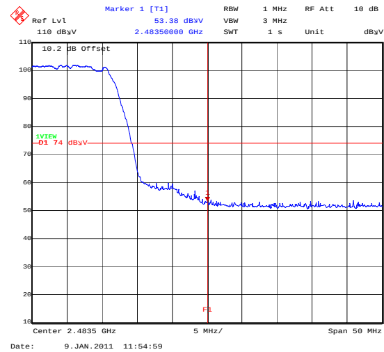
BandEdge_802_11G_24MBS_TopChannel
