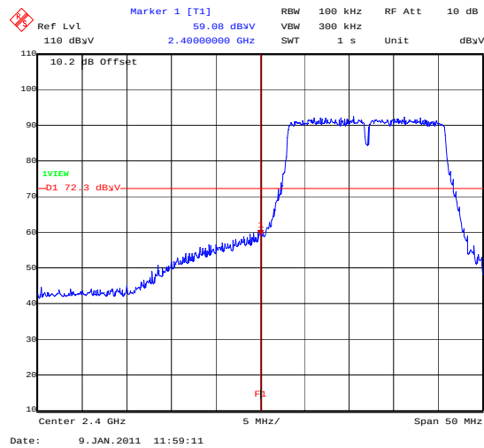
BandEdge_802_11N_6.5MBS_BotChannel
