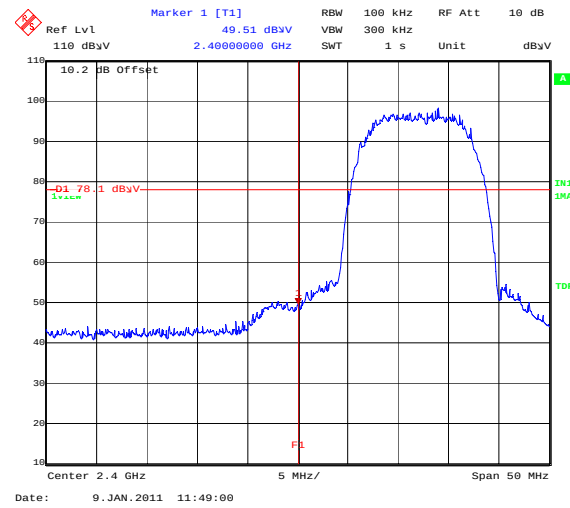
BandEdge_802_11B_11MBS_BotChannel
