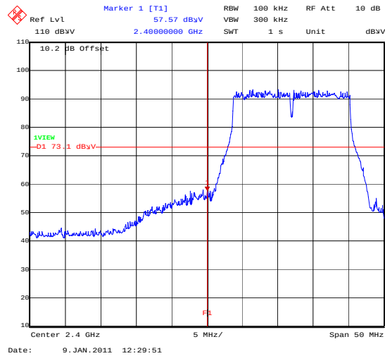
BandEdge_802_11G_48MBS_BotChannel
