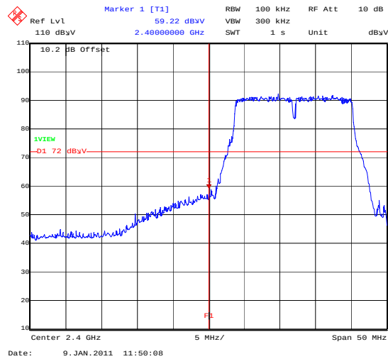
BandEdge_802_11G_6MBS_BotChannel
