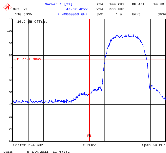
BandEdge_802_11B_5.5MBS_BotChannel
