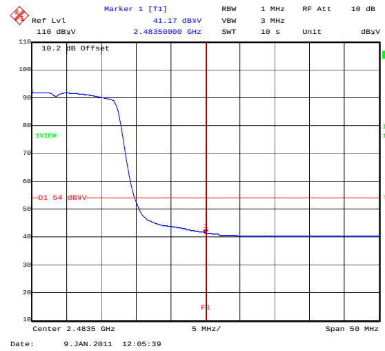
BandEdge_802_11N_52MBS_TopChannelAVG
