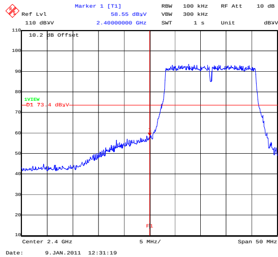
BandEdge_802_11N_58.5MBS_BotChannel
