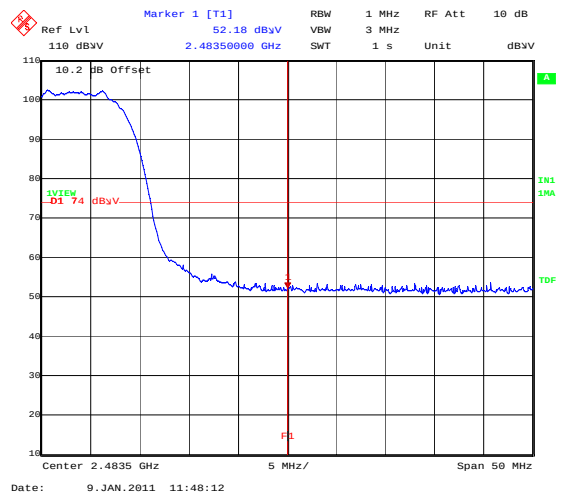
BandEdge_802_11B_5.5MBS_TopChannel
