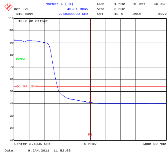
BandEdge_802_11G_9MBS_TopChannelAVG
