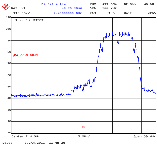
BandEdge_802_11B_1MBS_BotChannel
