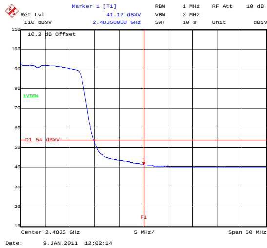
BandEdge_802_11N_19.5MBS_TopChannelAVG
