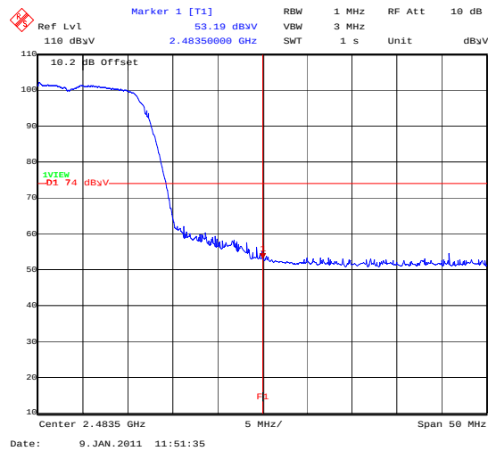
BandEdge_802_11G_9MBS_TopChannel
