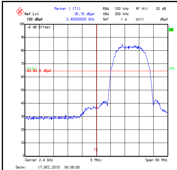
BandEdgeEIRP802_11B_5.5MBS_BottomChannel
