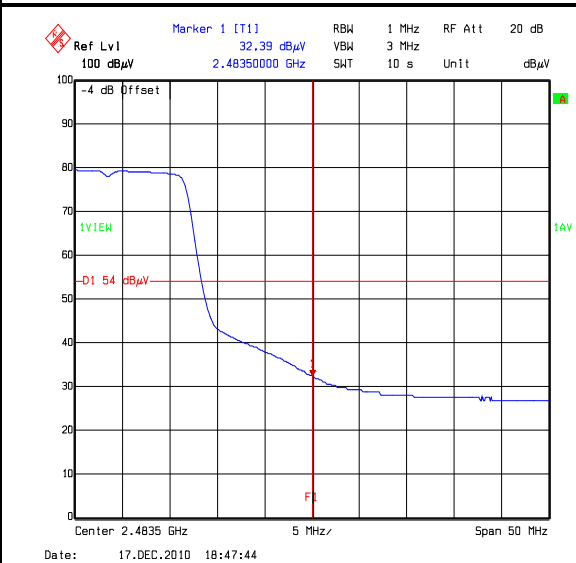
BandEdgeEIRP802_11G_18MBS_TopChannelAVG
