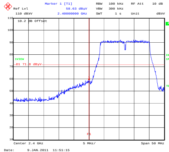
BandEdge_802_11G_9MBS_BotChannel
