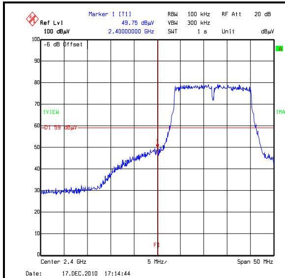
BandEdgeEIRP802_11G_18MBS_BottomChannel
