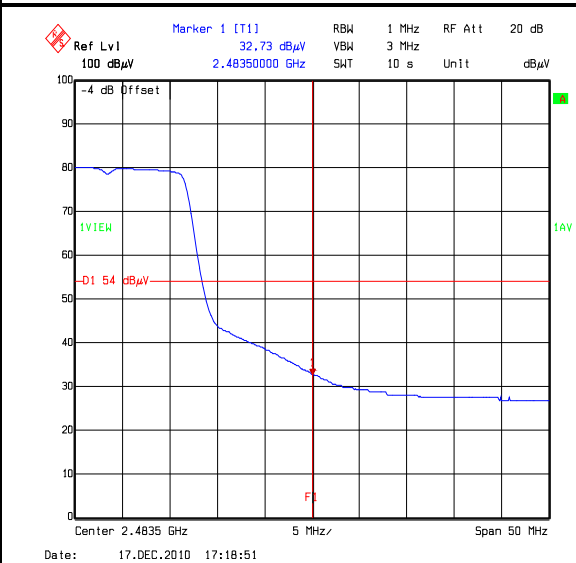
BandEdgeEIRP802_11G_36MBS_TopChannelAVG
