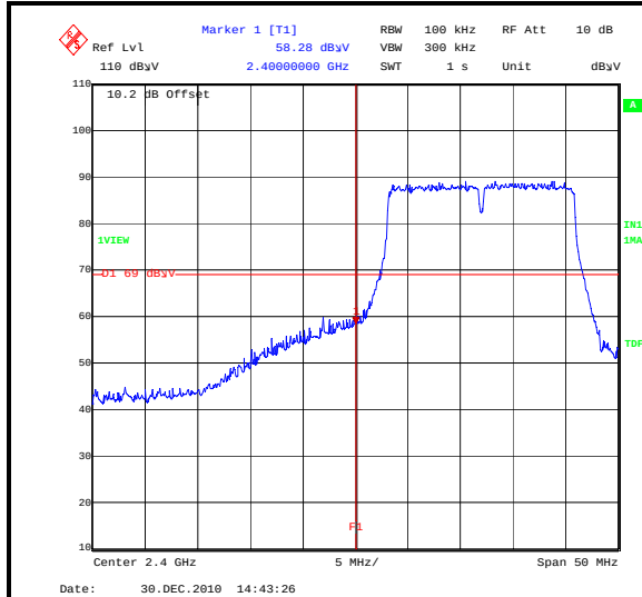
BandEdgeEIRP802_11N_13MBS_BotChannel
