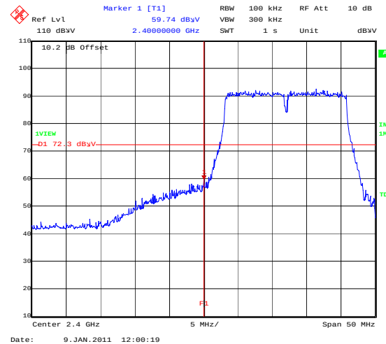
BandEdge_802_11N_13MBS_BotChannel
