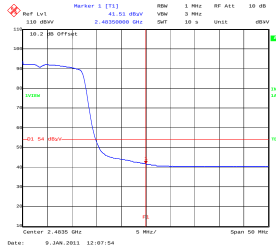
BandEdge_802_11N_65MBS_TopChannelAVG
