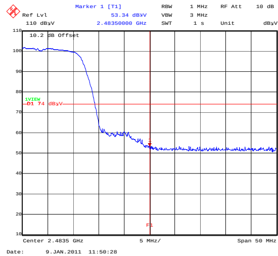
BandEdge_802_11G_6MBS_TopChannel
