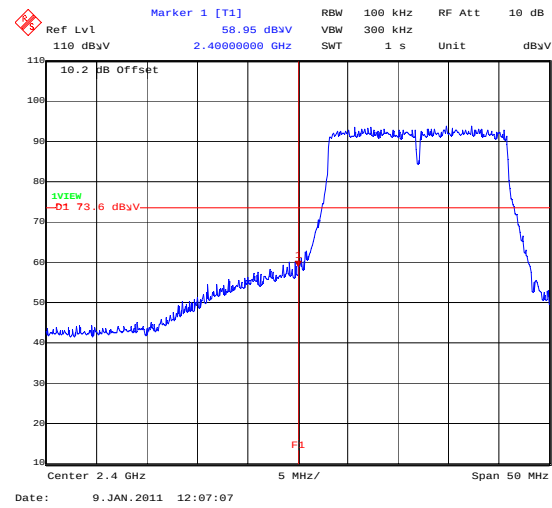
BandEdge_802_11N_65MBS_BotChannel
