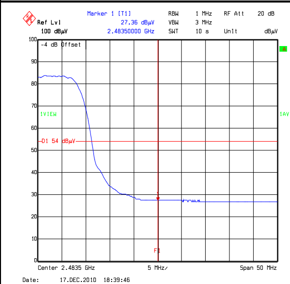
BandEdgeEIRP802_11B_5.5MBS_TopChannelAVG
