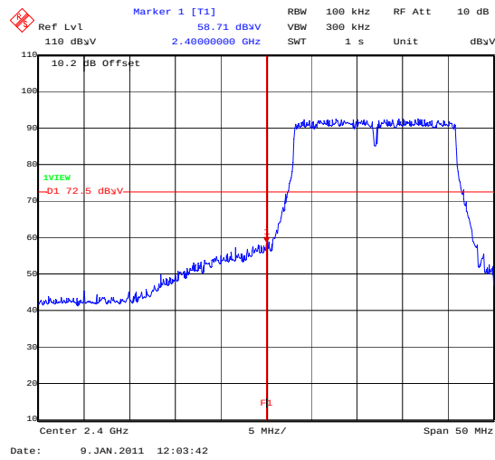
BandEdge_802_11N_39MBS_BotChannel
