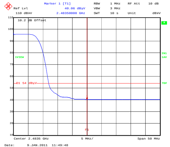
BandEdge_802_11B_11MBS_TopChannelAVG
