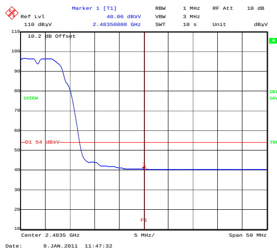
BandEdge_802_11B_2MBS_TopChannelAVG
