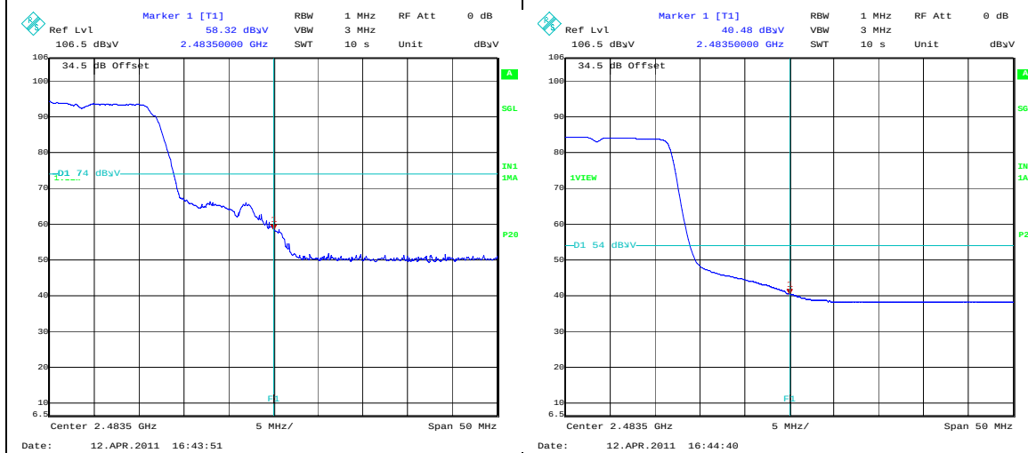
BandEdge-812.11g-9Mbps-Top-Peak
