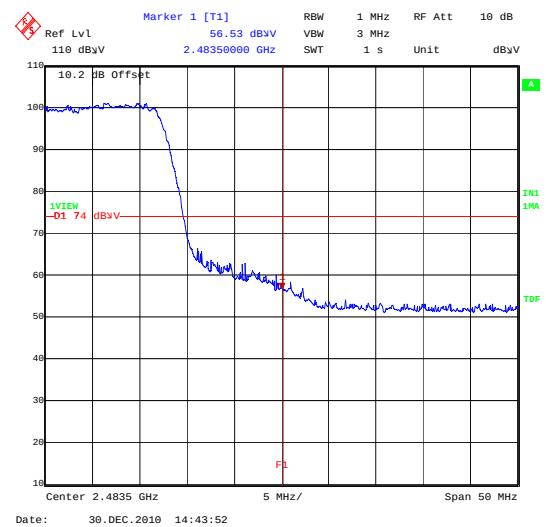
BandEdgeEIRP802_11N_13MBS_TopChannelAVG
