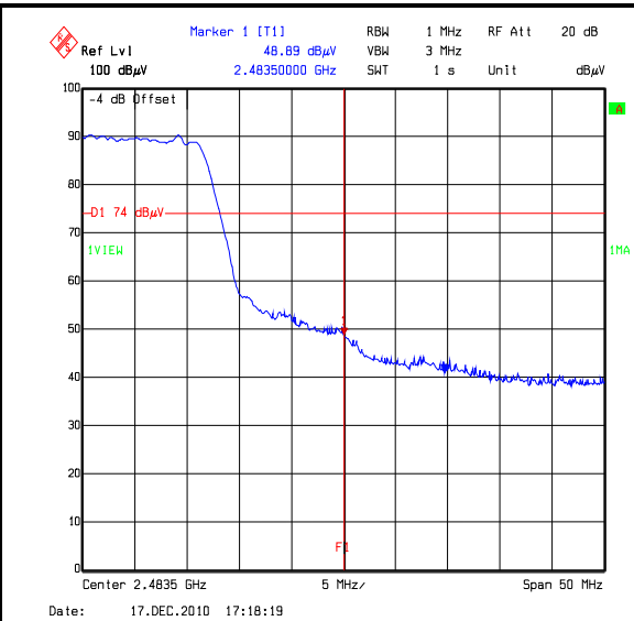
BandEdgeEIRP802_11G_36MBS_TopChannel
