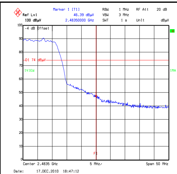
BandEdgeEIRP802_11G_18MBS_TopChannel
