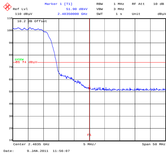
BandEdge_802_11G_36MBS_TopChannel
