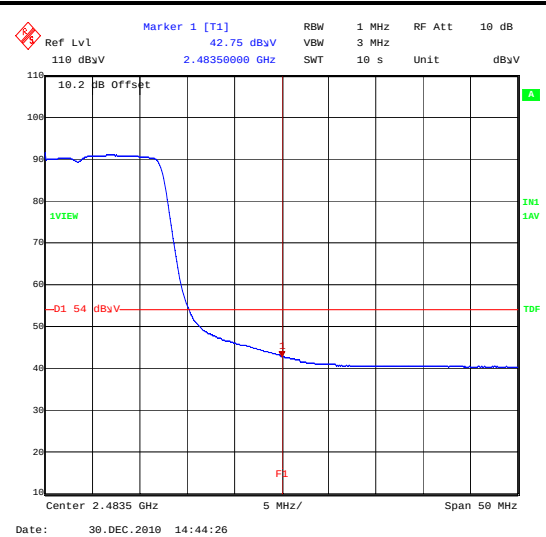
BandEdgeEIRP802_11N_13MBS_TopChannel
