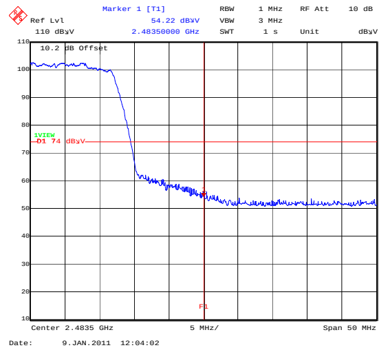
BandEdge_802_11N_39MBS_TopChannel
