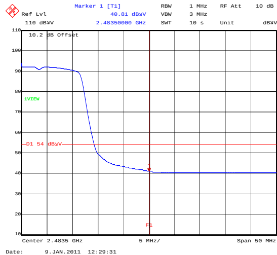
BandEdge_802_11G_6MBS_TopChannelAVG
