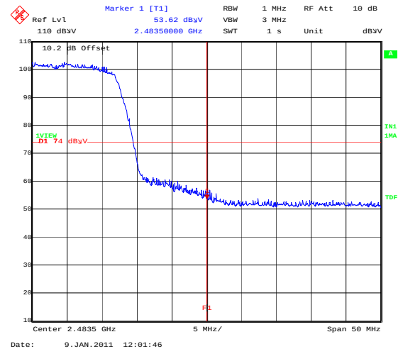
BandEdge_802_11N_19.5MBS_TopChannel
