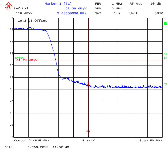
BandEdge_802_11G_12MBS_TopChannel
