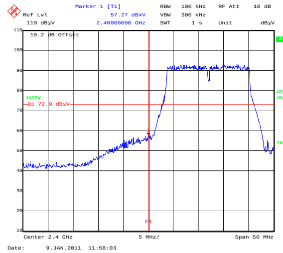
BandEdge_802_11G_54MBS_BotChannel
