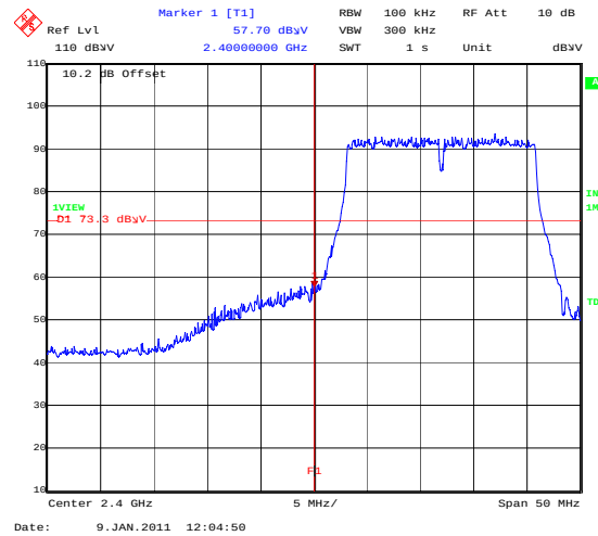
BandEdge_802_11N_52MBS_BotChannel
