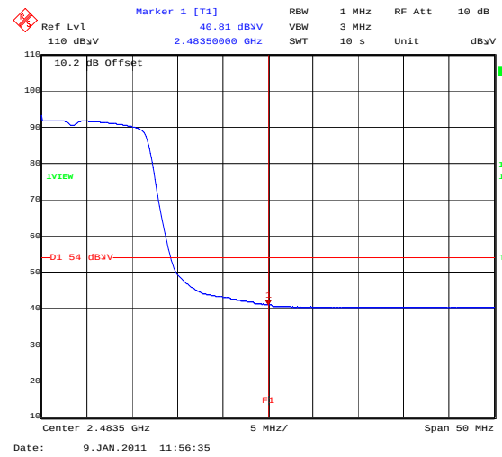
BandEdge_802_11G_36MBS_TopChannelAVG
