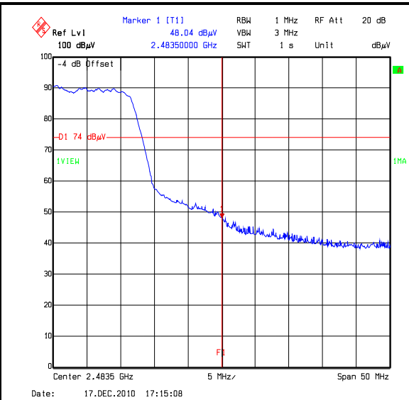
BandEdgeEIRP802_11G_18MBS_TopChannel
