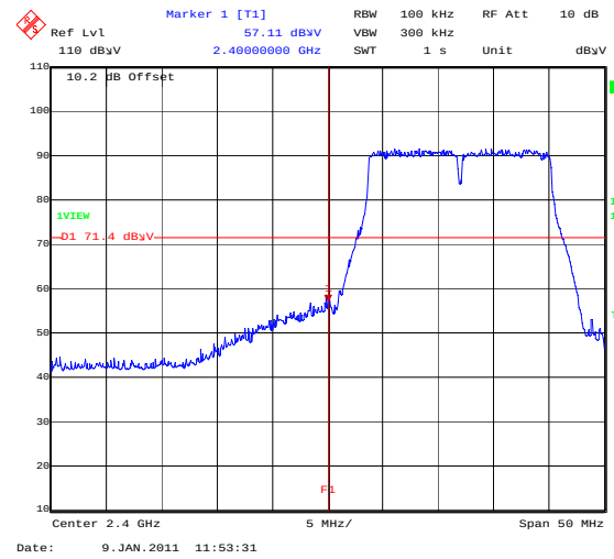
BandEdge_802_11G_18MBS_BotChannel
