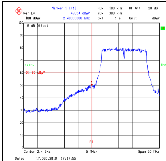
BandEdgeEIRP802_11G_36MBS_BottomChannel
