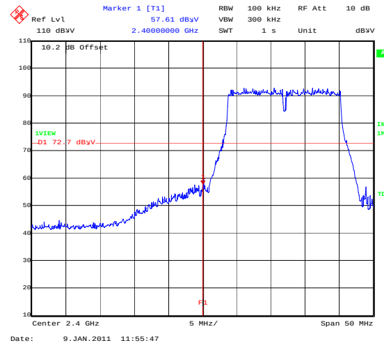
BandEdge_802_11G_36MBS_BotChannel
