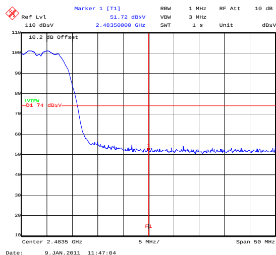
BandEdge_802_11B_2MBS_TopChannel
