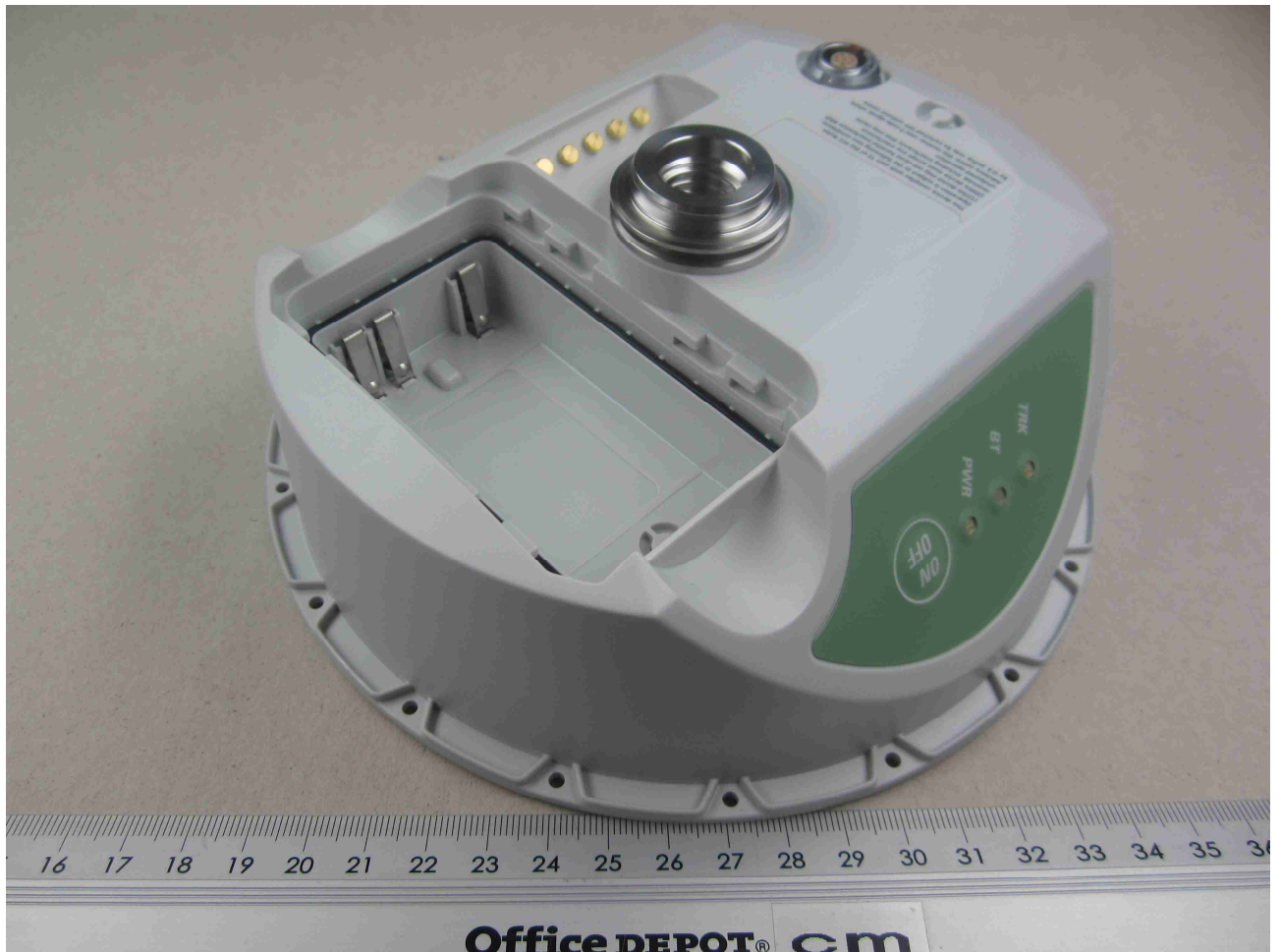
130857_25.JPG: EUT/antenna housing, top view 1, battery removed
