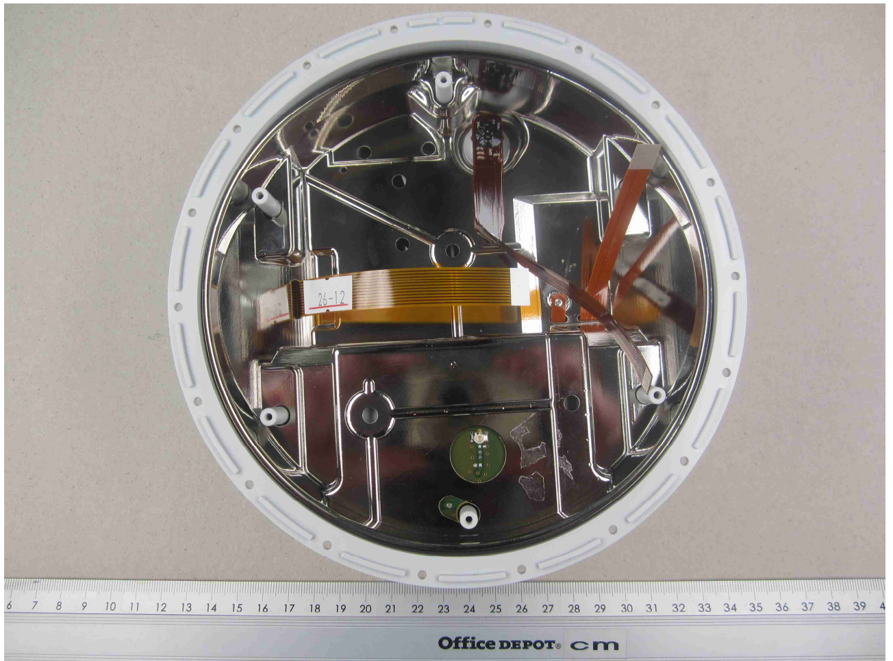
130857_12.JPG: EUT/antenna housing, bottom view
