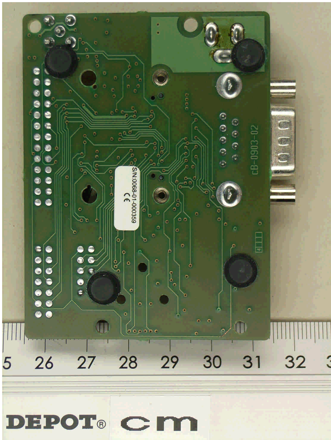
101347_c.jpg: cB-0903-02, carrier board, bottom view
