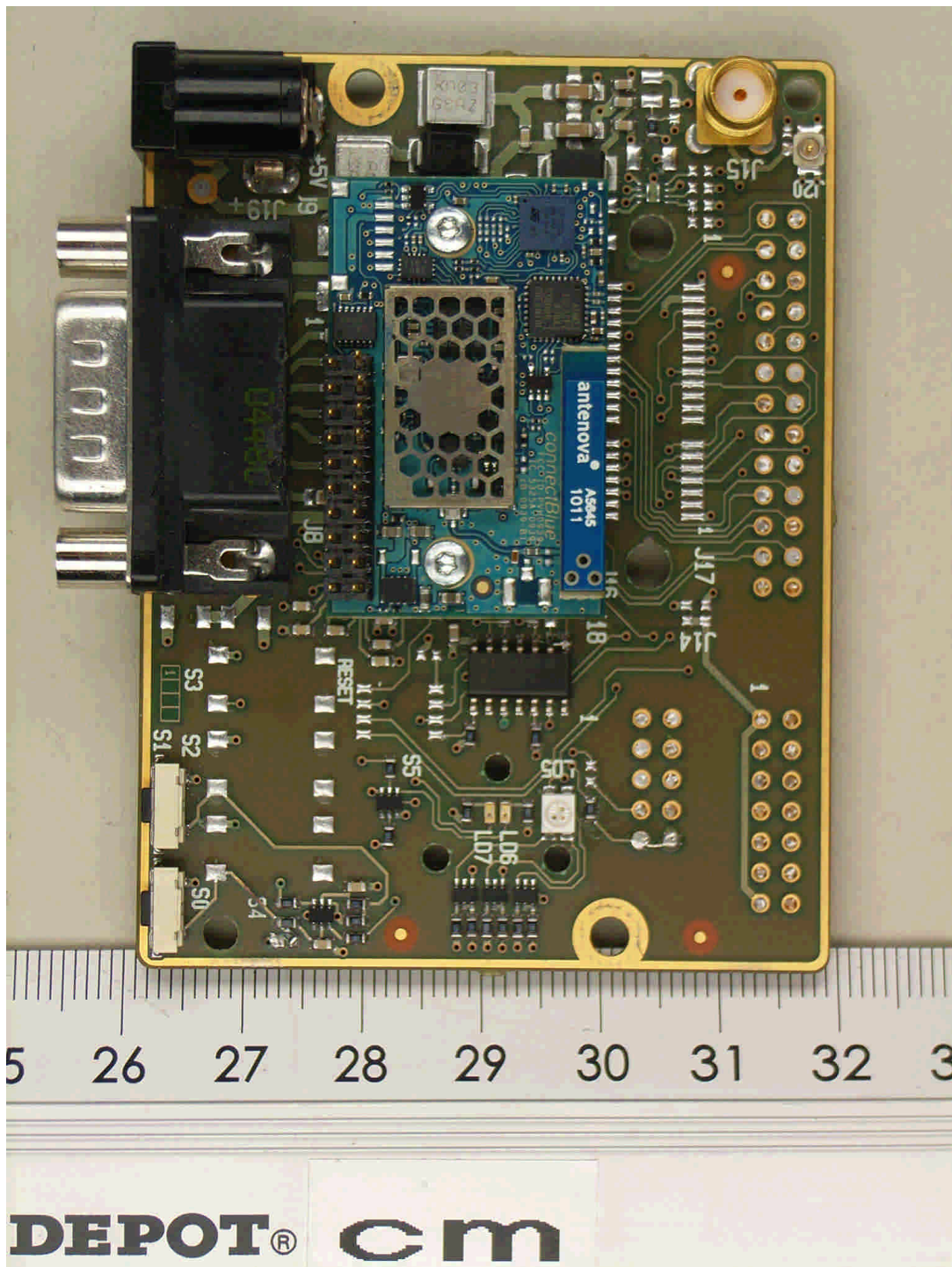
101347_a.jpg: cB-0903-02, carrier board, top view
