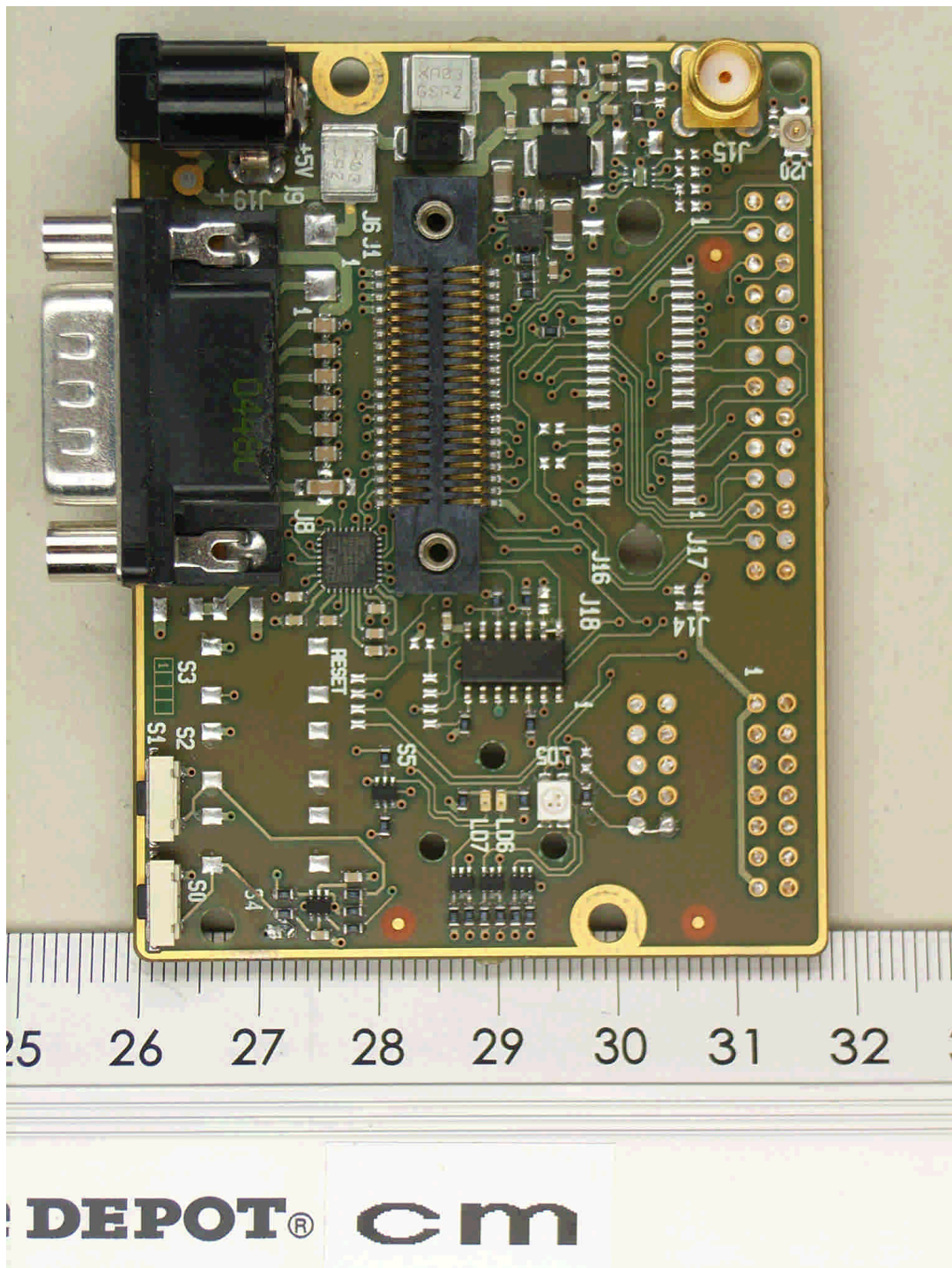
101347_b.jpg: cB-0903-02, carrier board, top view, module removed
