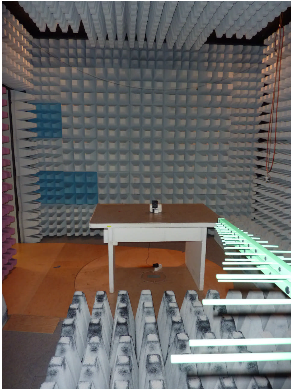
112117_4.JPG: cB-0939 with EPA antenna, test setup fully anechoic chamber
