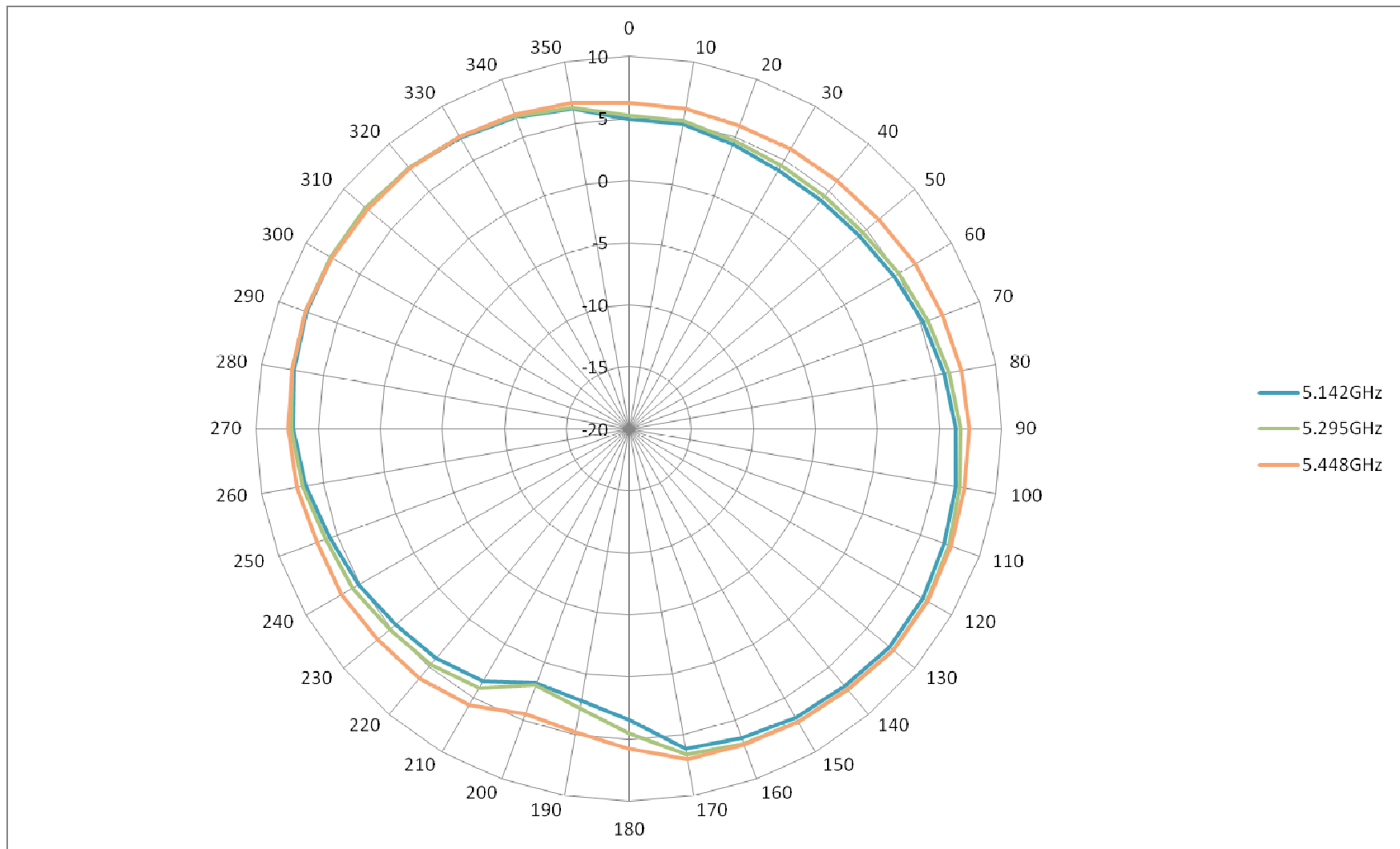
Figure 1 – Radiation pattern straight forward
