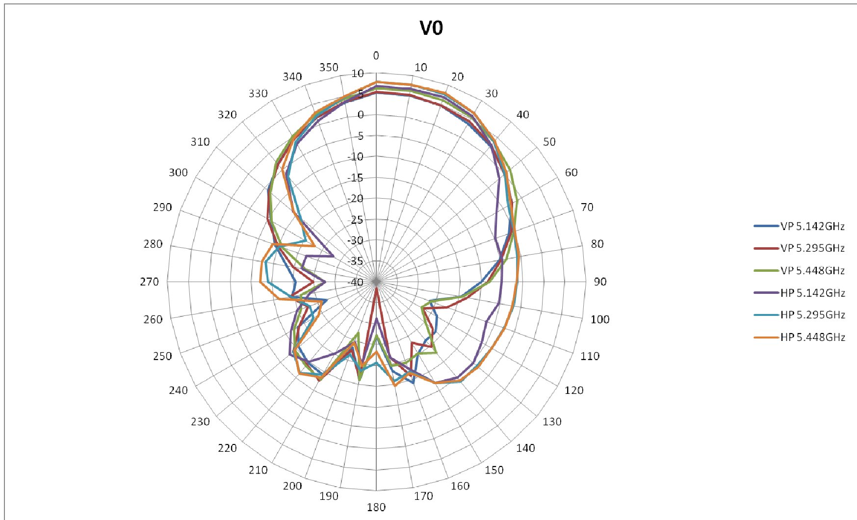
Figure 2 - Radiation pattern of the 5Ghz antenna
