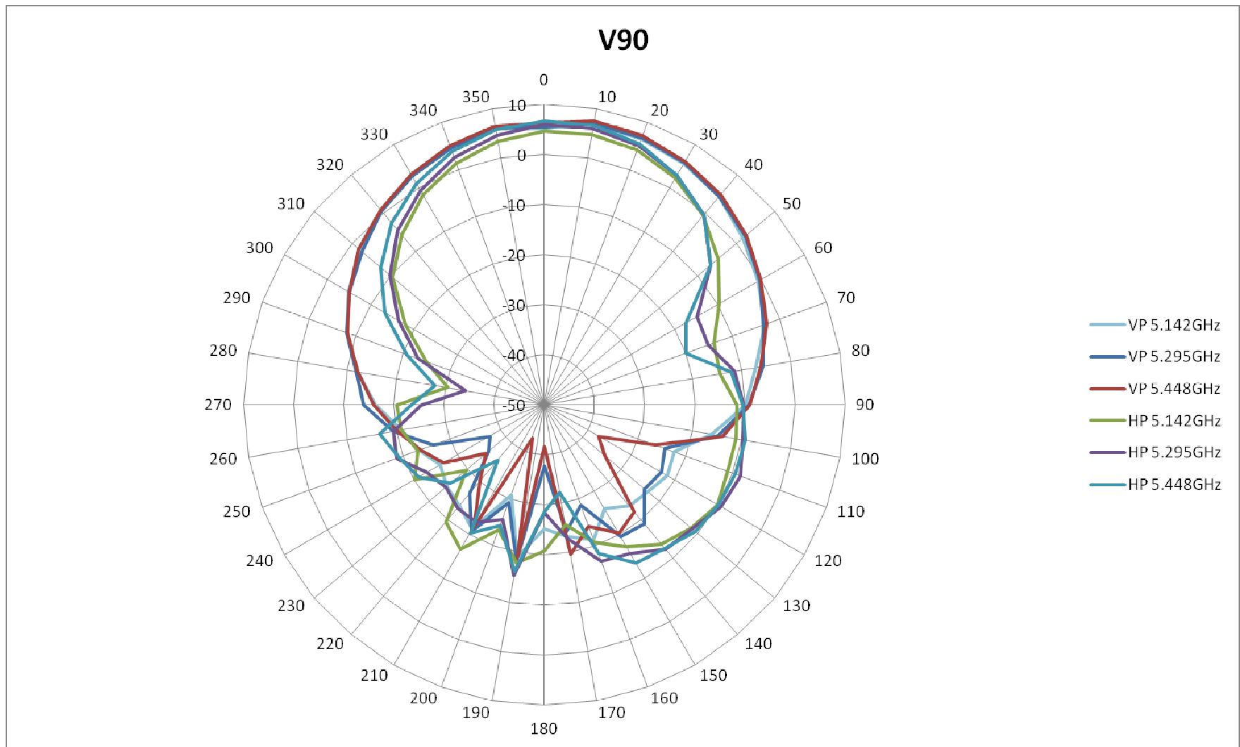
Figure 3 - Radiation pattern of the 5Ghz antenna
