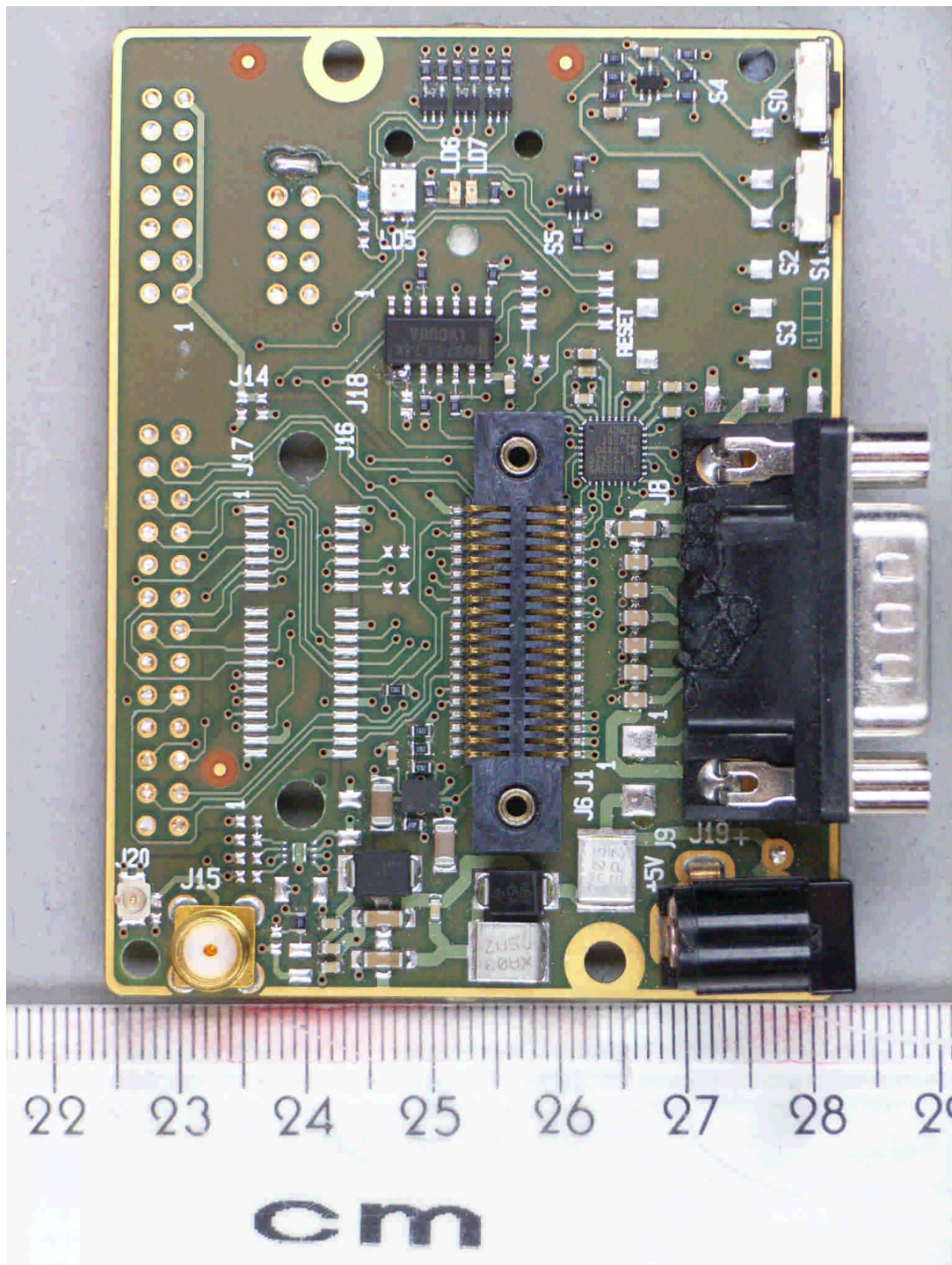
103572_b.jpg cB-0903-02, carrier board, top view
