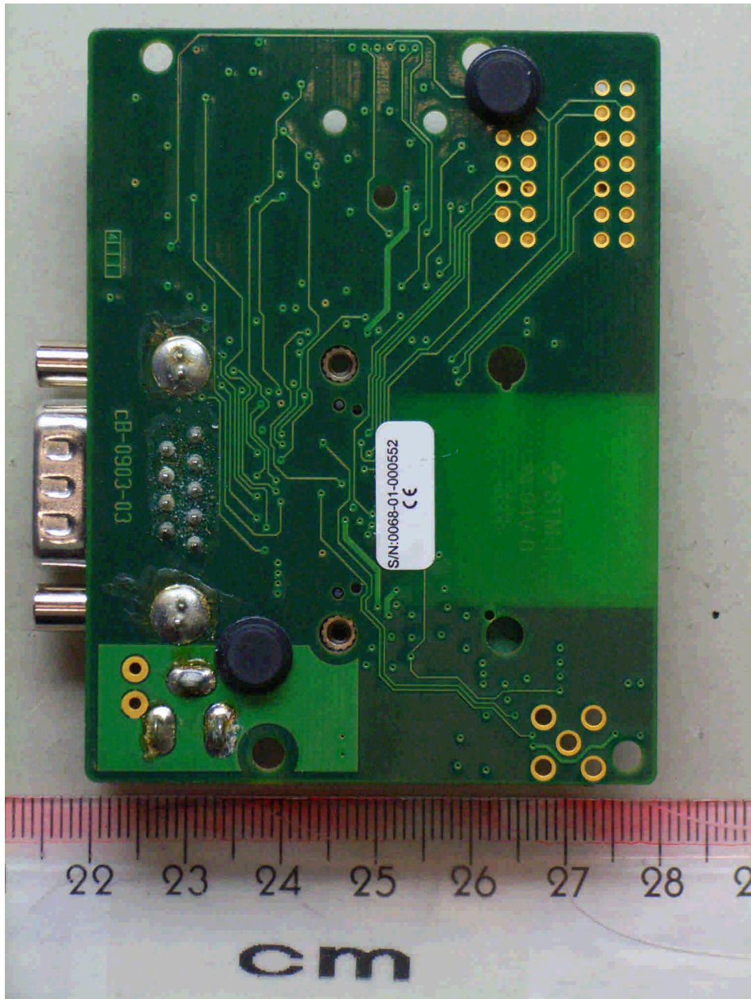
82155_12.jpg cB-0903-03 carrier board, bottom view
