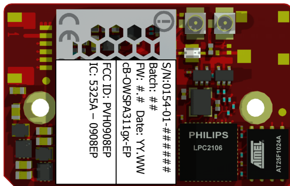
Figure 1 OWSPA311gx-EP Serial label and FCC ID/IC label
