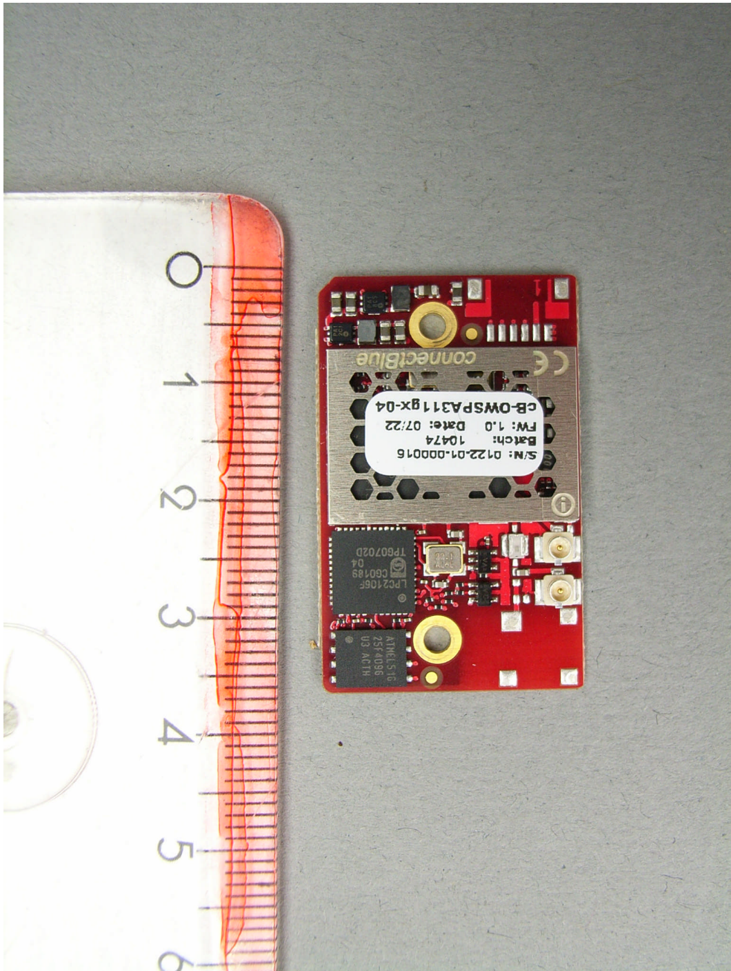
71312PCB4.JPG Radio board front view
