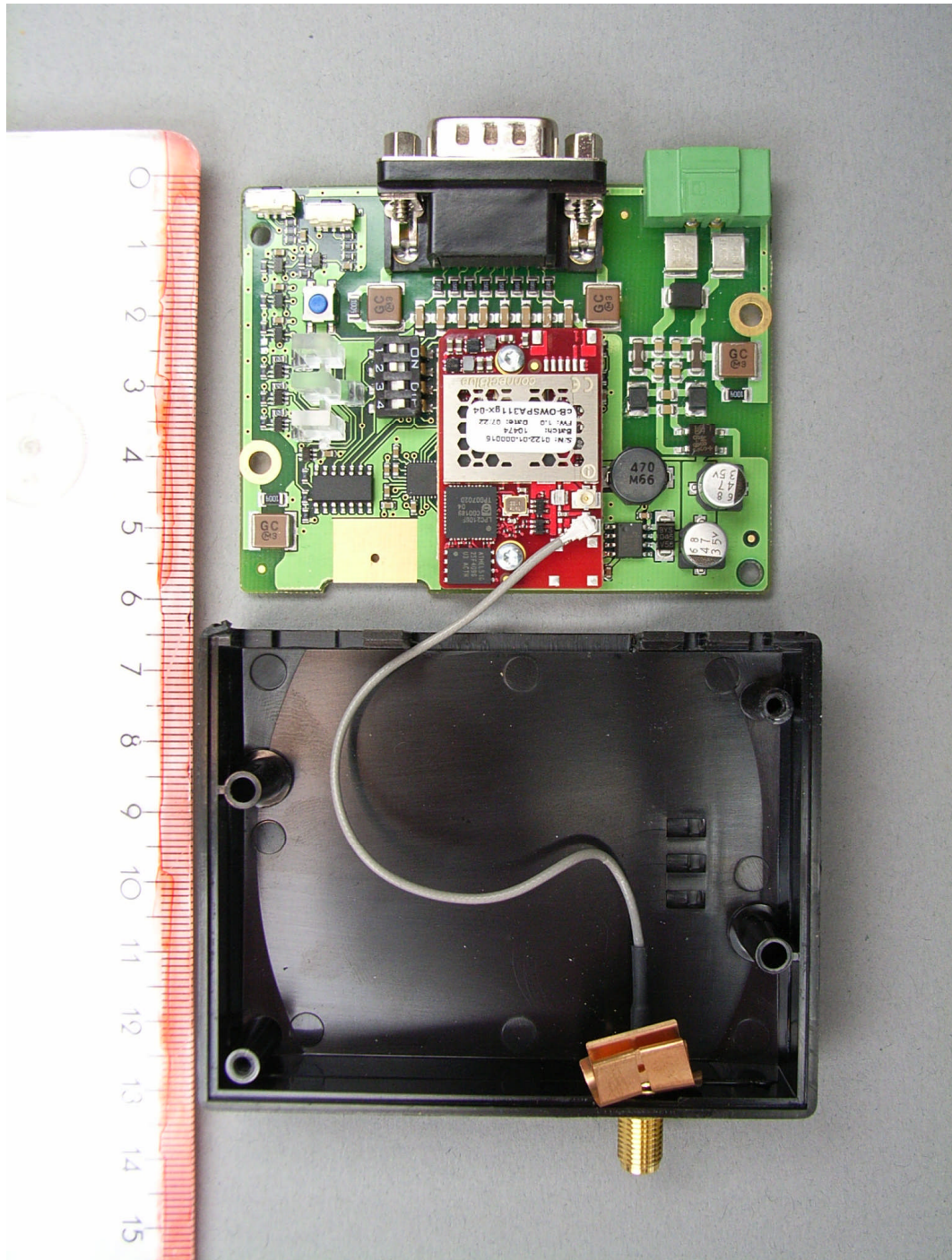
71312PCB2.JPG Main board front view
