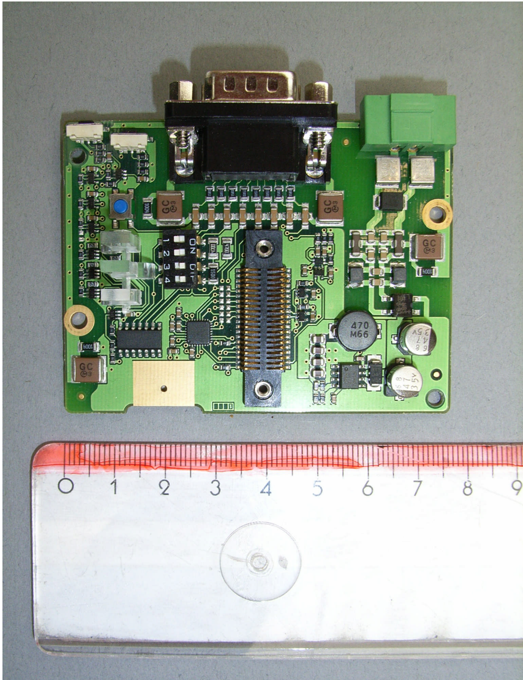
71312PCB3.JPG Main board front view, radio board disassembled
