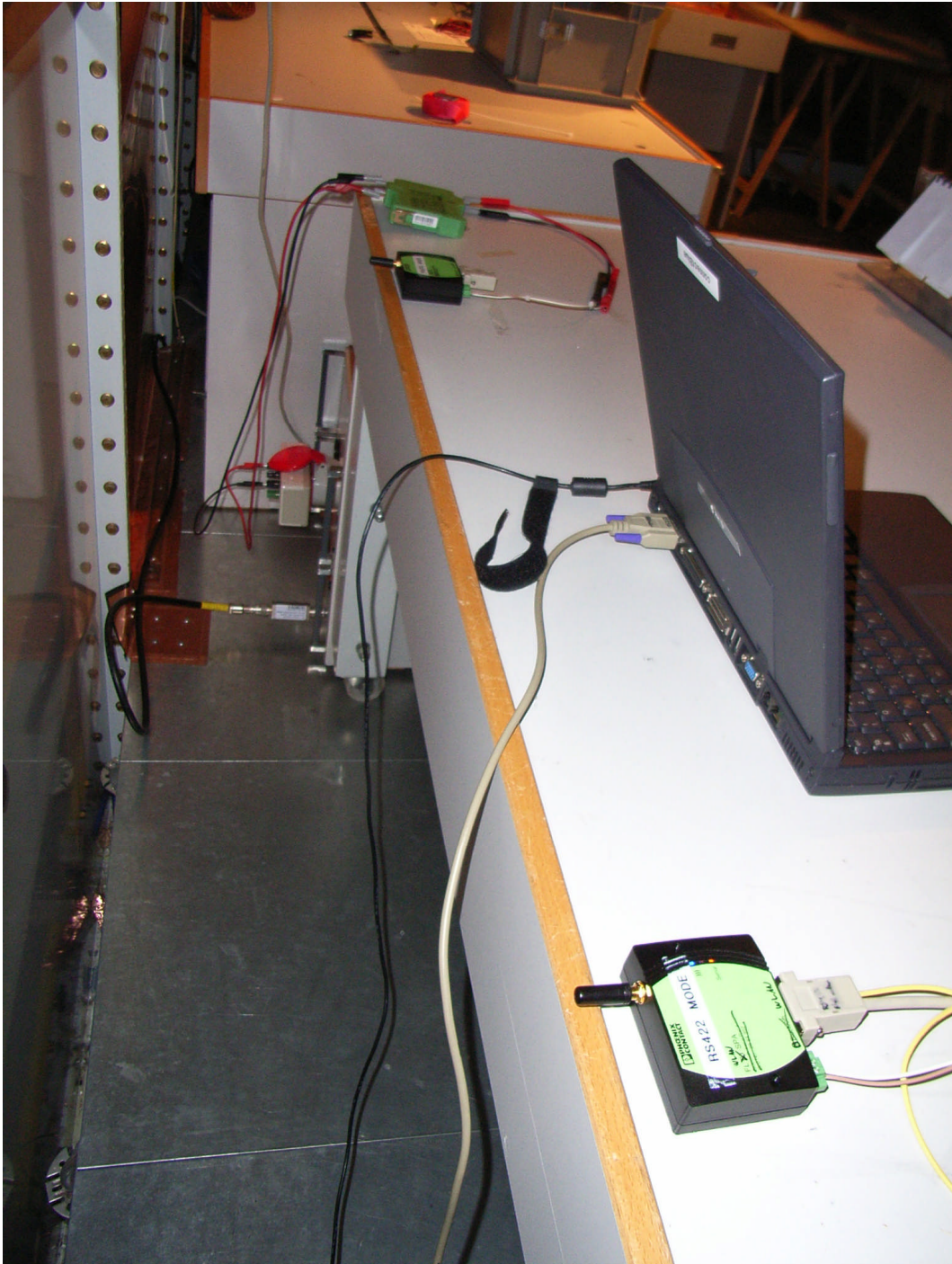
71312AC232_2.jpg Test set-up conducted emission measurement
