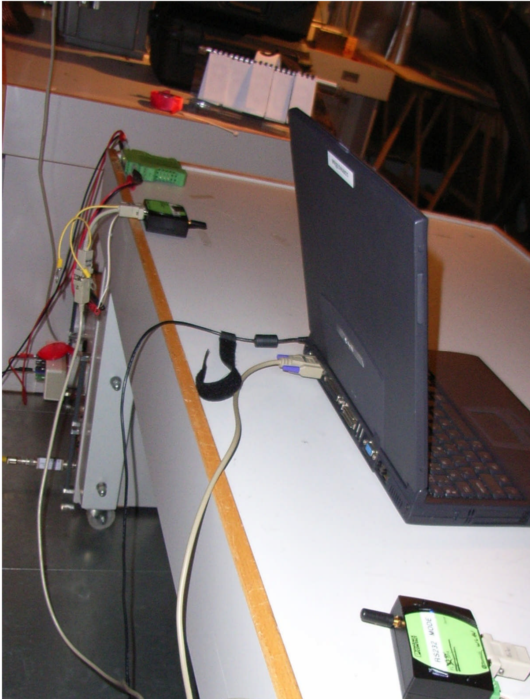
71312AC485_2.jpg Test set-up conducted emission measurement
