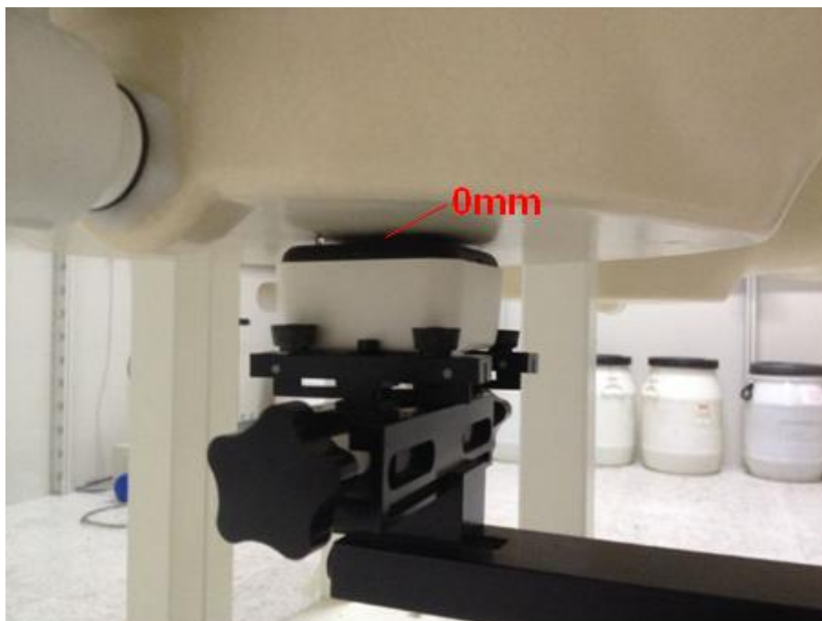
WIFI SAR Back face 0mm for Head
