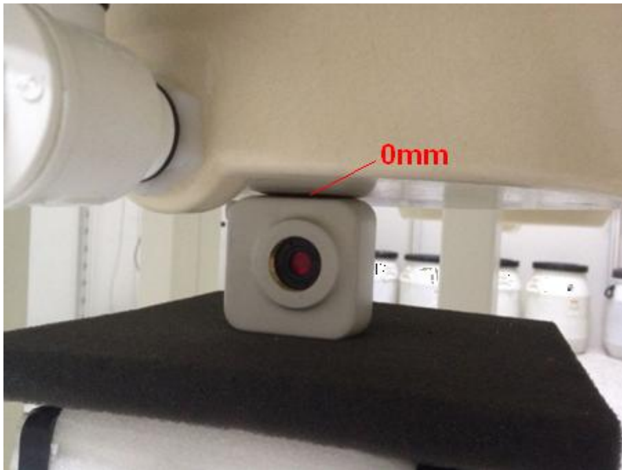
WIFI SAR Bottom face 0mm for Head
