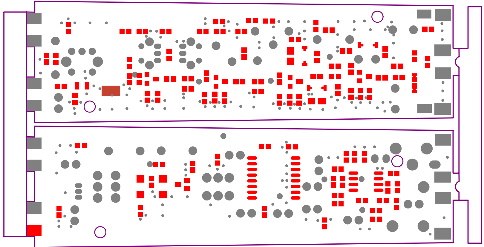
HT-U20 Transmitter Top Solder and Paste Mask
