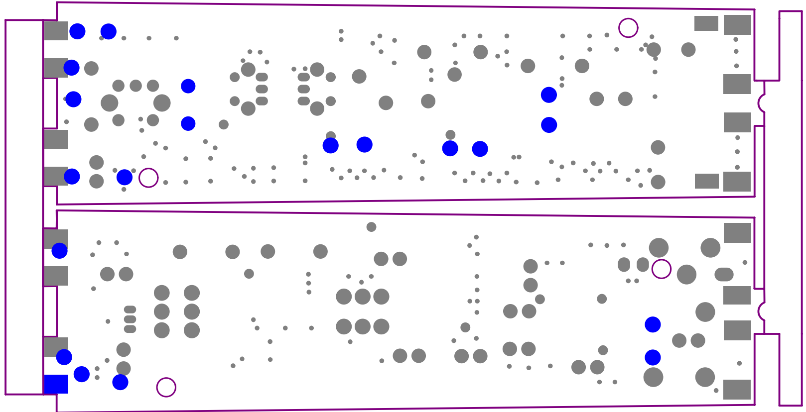
HT-U20 Transmitter Bottom Solder and Paste Mask
