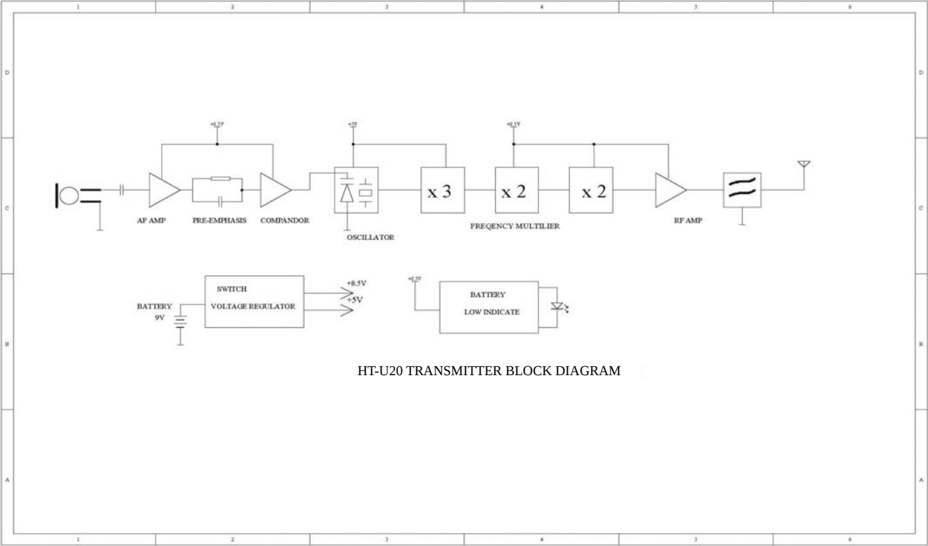
HT-U20 Block Diagram
