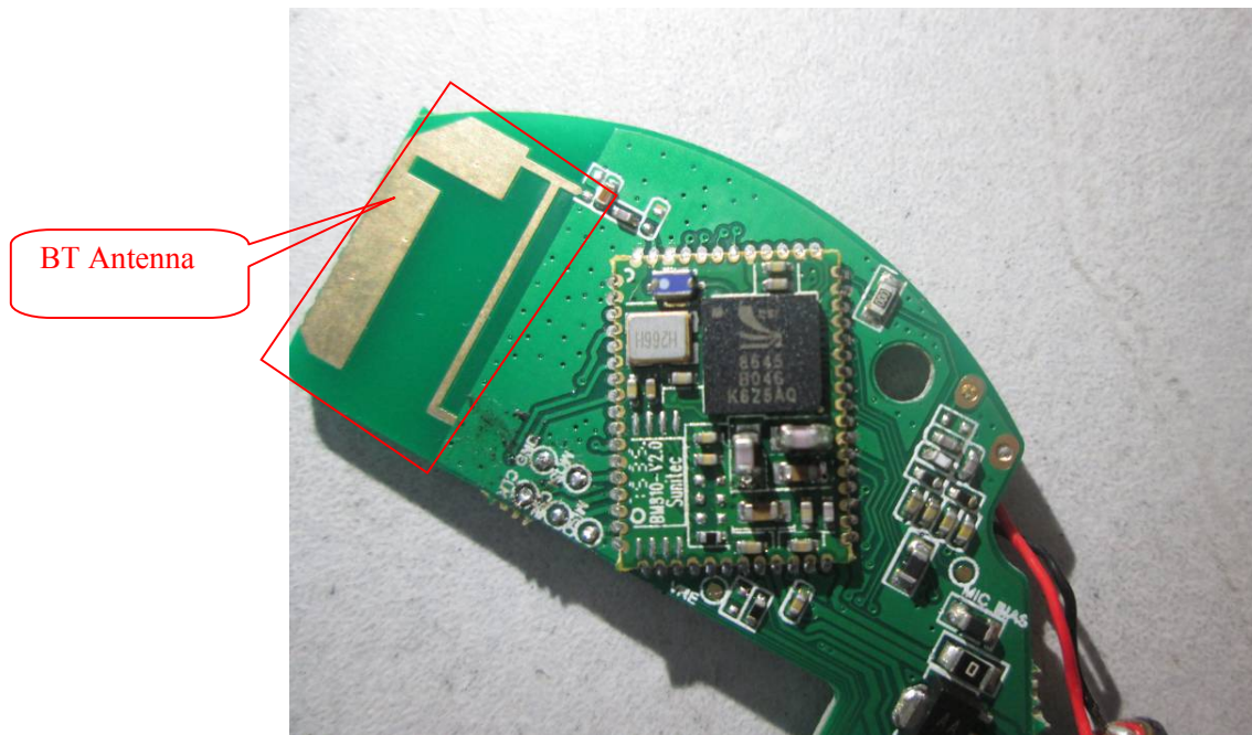
EUT – IC Chip 1 View
