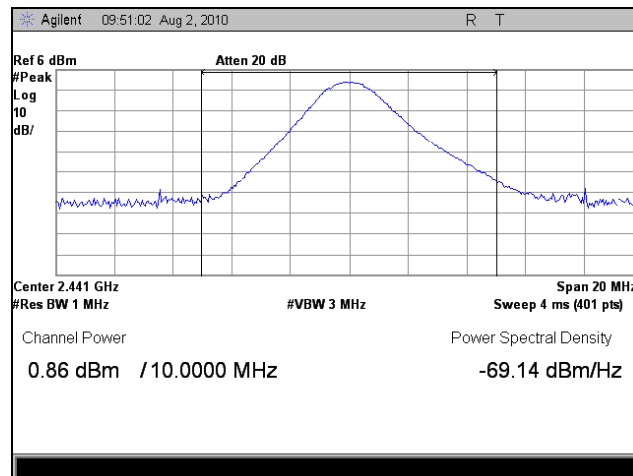
Plot 15. Peak Output Power, Mid Channel, Channel Integration
