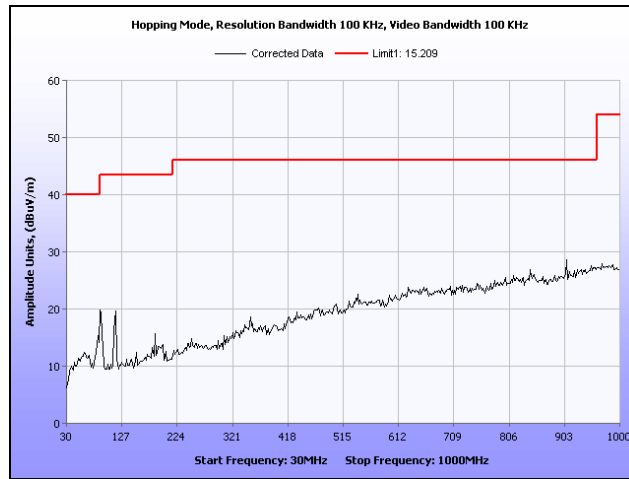
Plot 23. Radiated Spurious Emissions, Hopping Mode, 30 MHz – 1 GHz
