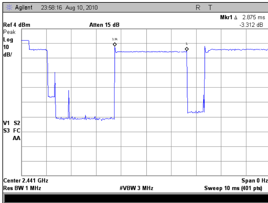
Plot 13. Time Occupancy
