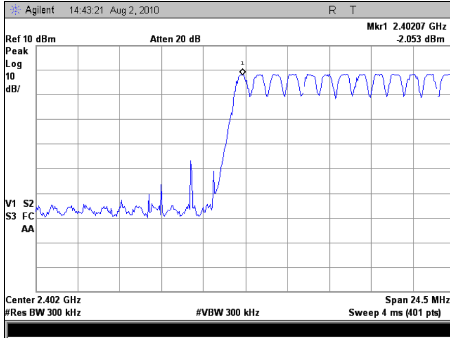
Plot 9. Bottom Half of Frequency Range, 1
