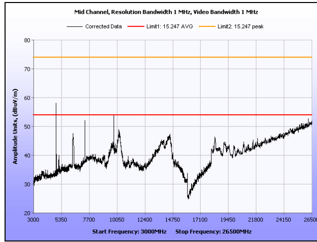
Plot 20. Radiated Spurious Emissions, Mid Channel, 3 GHz – 26.5 GHz
