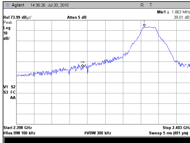
Plot 29. 20dBc Requirement, Low Channel
