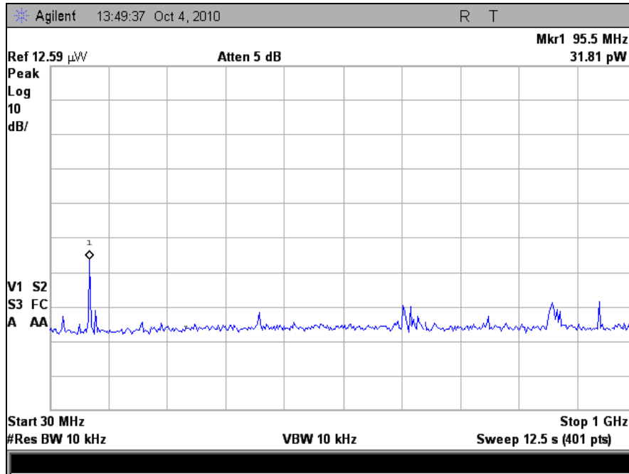
Plot 35. Receiver Spurious Emission, 30 MHz – 1 GHz
