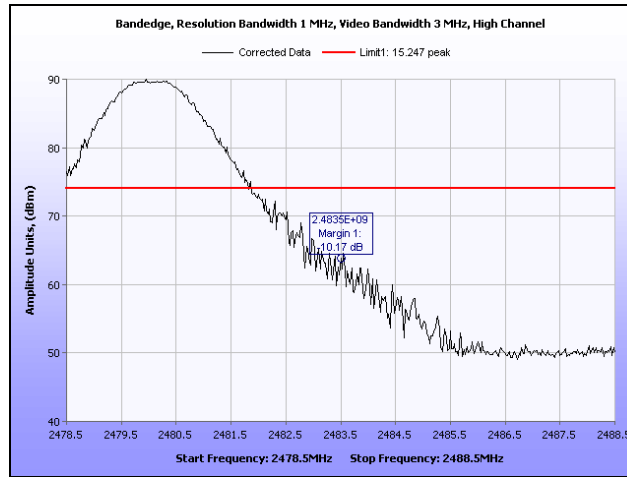
Plot 28. Radiated Restricted Band Edge, High Chanel, Peak
