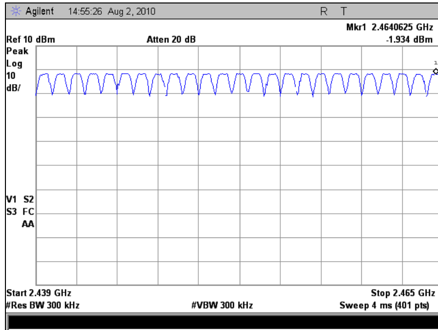
Plot 11. Top Half of Frequency Range, 1
