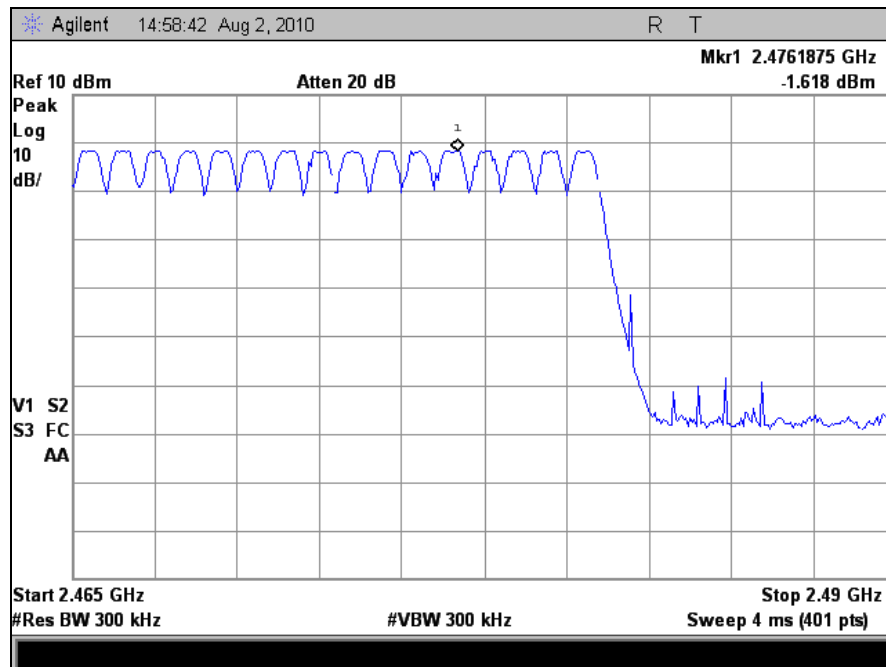
Plot 12. Top Half of Frequency Range, 2
