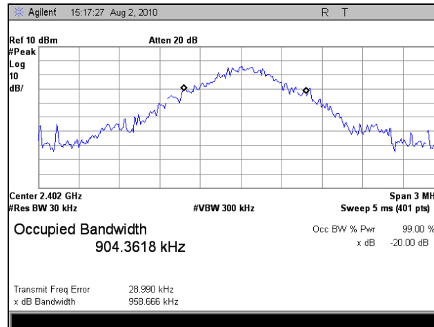
Plot 5. Occupied Bandwidth, Low Channel
