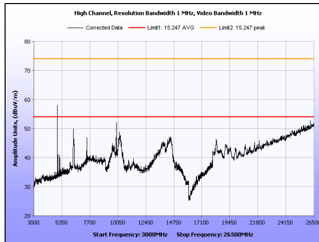
Plot 22. Radiated Spurious Emissions, High Channel, 3 GHz – 26.5 GHz
