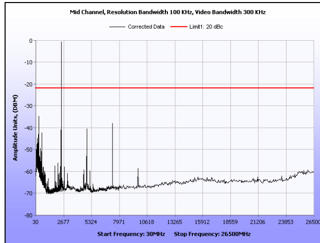
Plot 32. Conducted Spurious Emissions, Mid Channel
