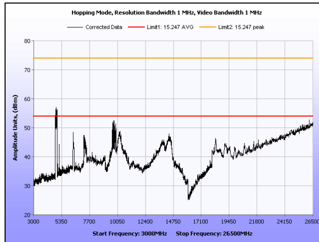
Plot 24. Radiated Spurious Emissions, Hopping Mode, 3 GHz – 26.5 GHz
