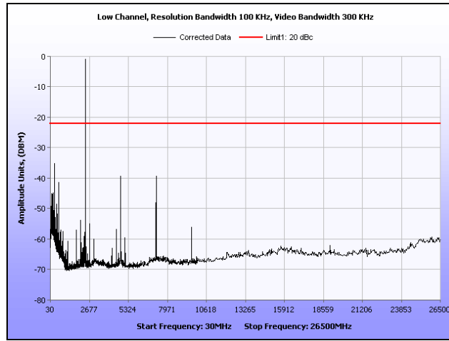
Plot 31. Conducted Spurious Emissions, Low Channel
