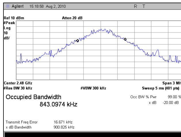
Plot 7. Occupied Bandwidth, High Channel
