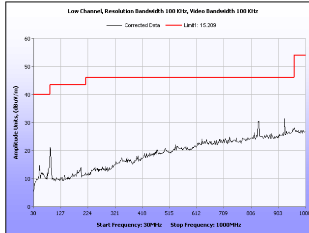
Plot 17. Radiated Spurious Emissions, Low Channel, 30 MHz – 1 GHz
