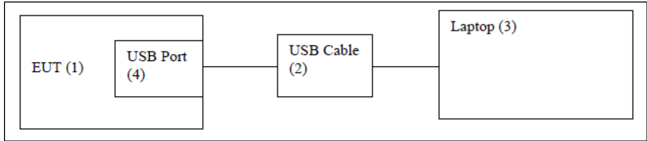
Figure 1. Block Diagram of Test Configuration, Mode 1
