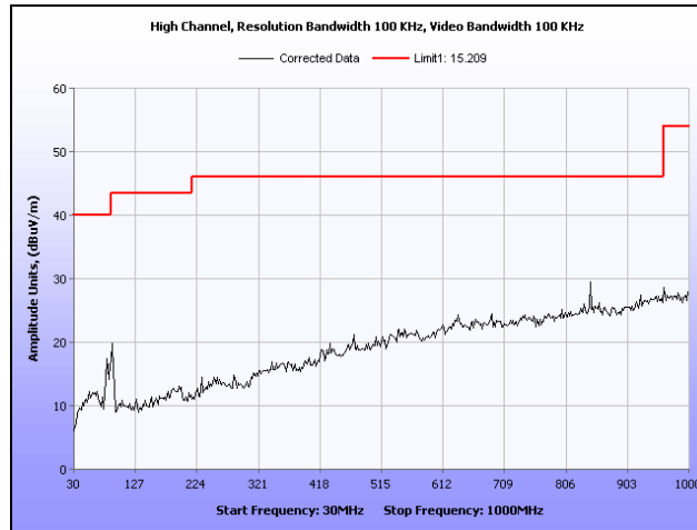
Plot 21. Radiated Spurious Emissions, High Channel, 30 MHz – 1 GHz
