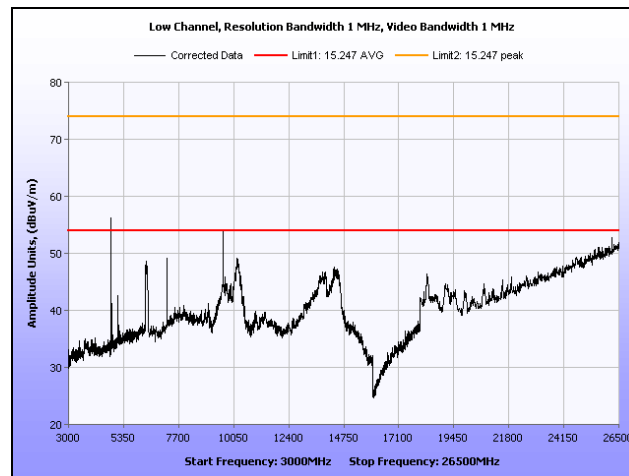
Plot 18. Radiated Spurious Emissions, Low Channel, 3 GHz – 26.5 GHz
