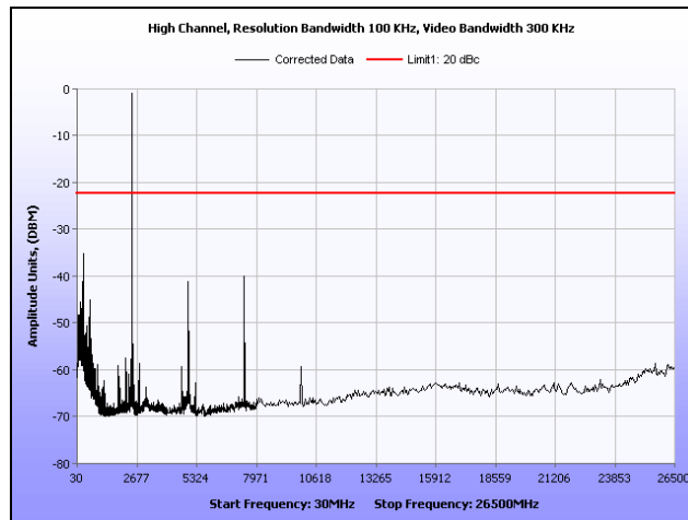
Plot 33. Conducted Spurious Emissions, High Channel
