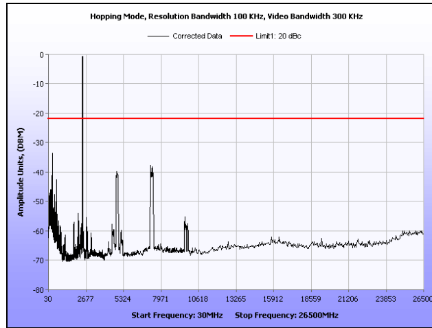
Plot 34. Conducted Spurious Emissions, Hopping Mode
