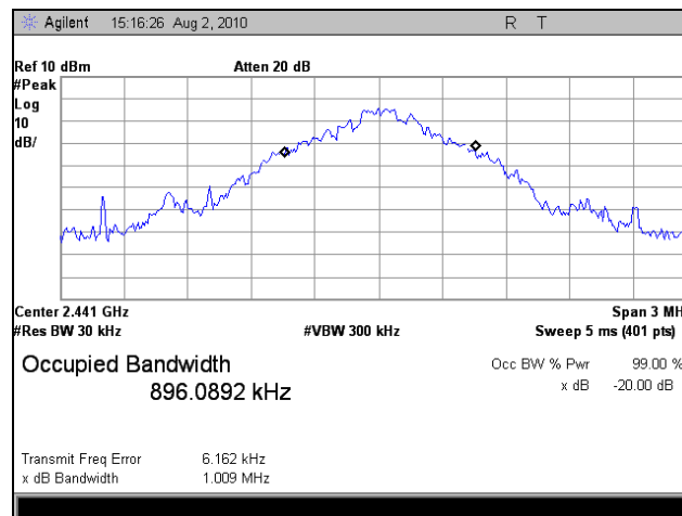
Plot 6. Occupied Bandwidth, Mid Channel
