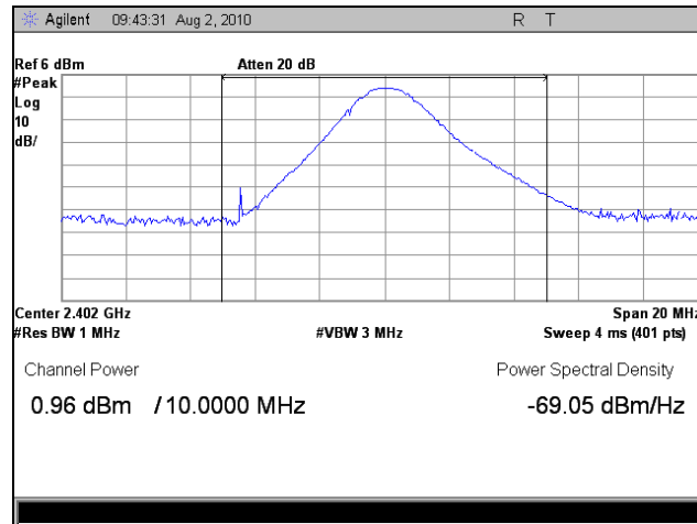
Plot 14. Peak Output Power, Low Channel, Channel Integration
