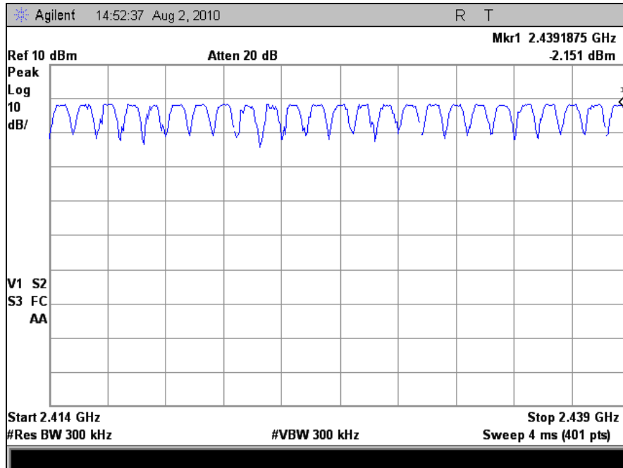
Plot 10. Bottom Half of Frequency Range, 2
