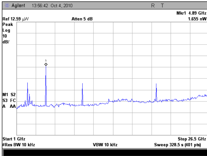
Plot 36. Receiver Spurious Emission, 1 GHz – 26.5 GHz
