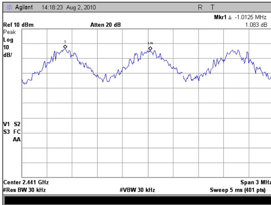
Plot 8. Channel Separation
