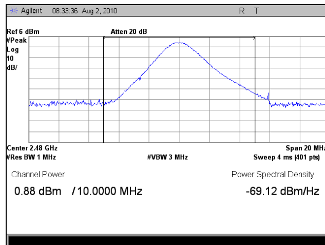
Plot 16. Peak Output Power, High Channel, Channel Integration
