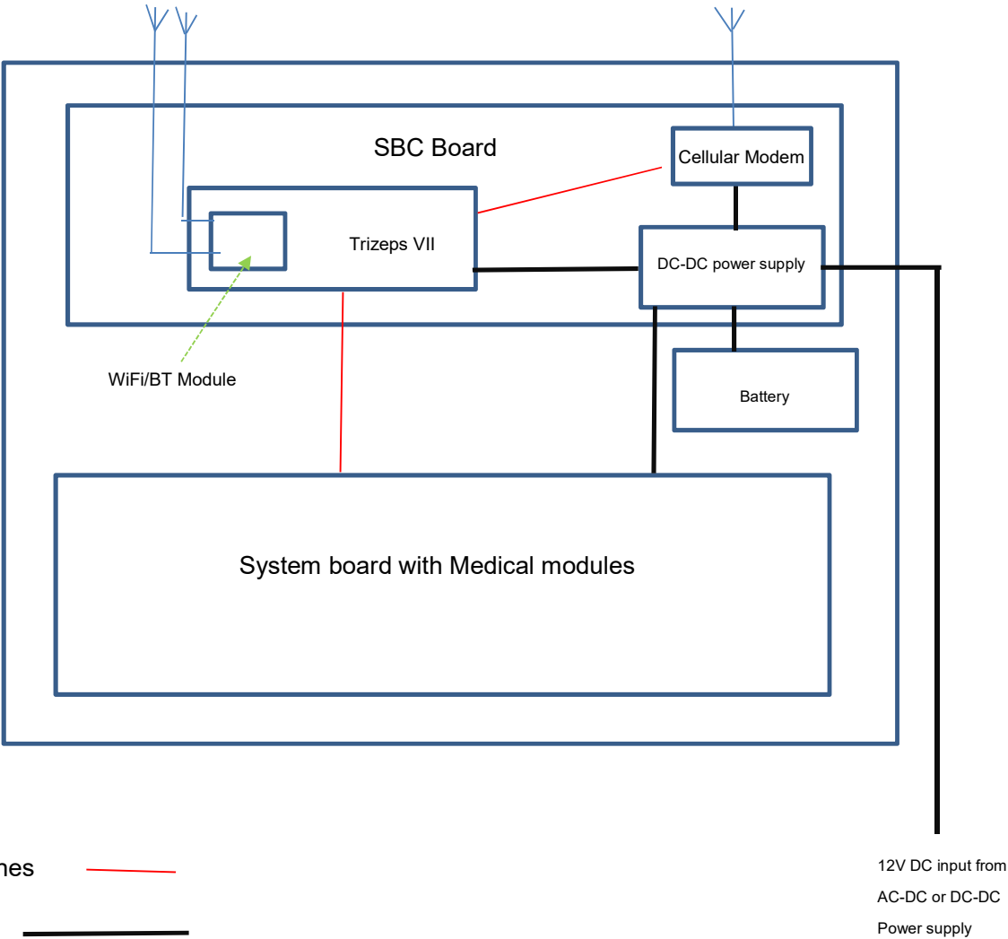
Tempus Pro Simplified block diagram
