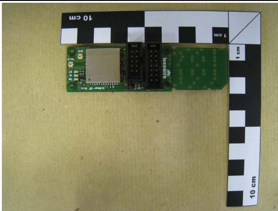
WiBear-SF2 Top with shieldings
