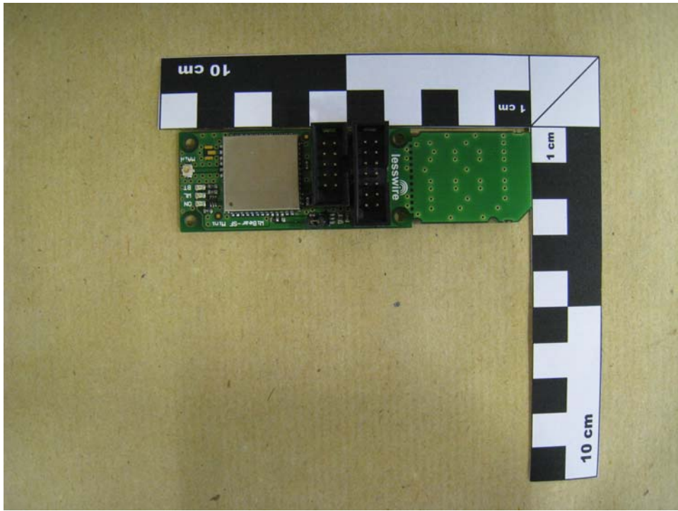
WiBear-SF1 Top with shieldings
