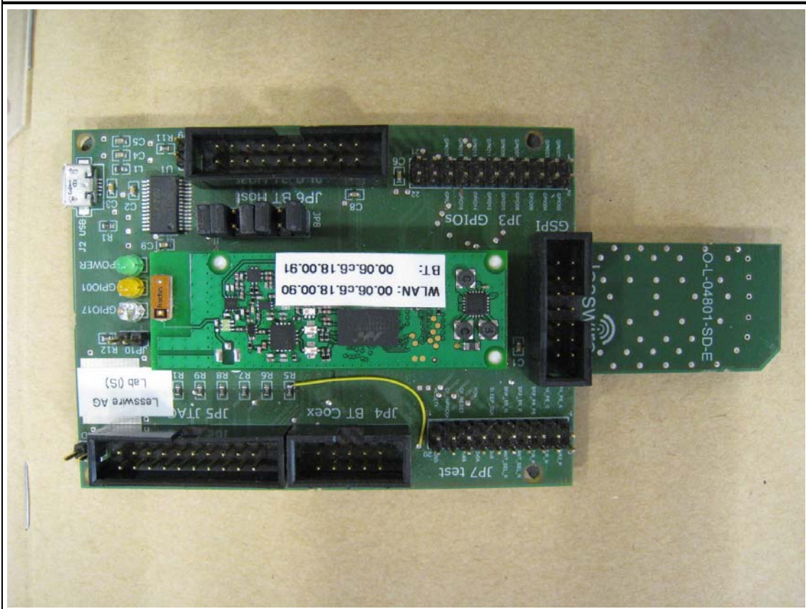
WiBear-I with evaluation board
