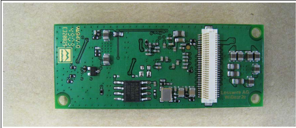
WiBear-E Bottom without shieldings
