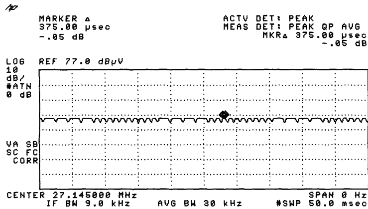
Figure C [Short Pulse]
