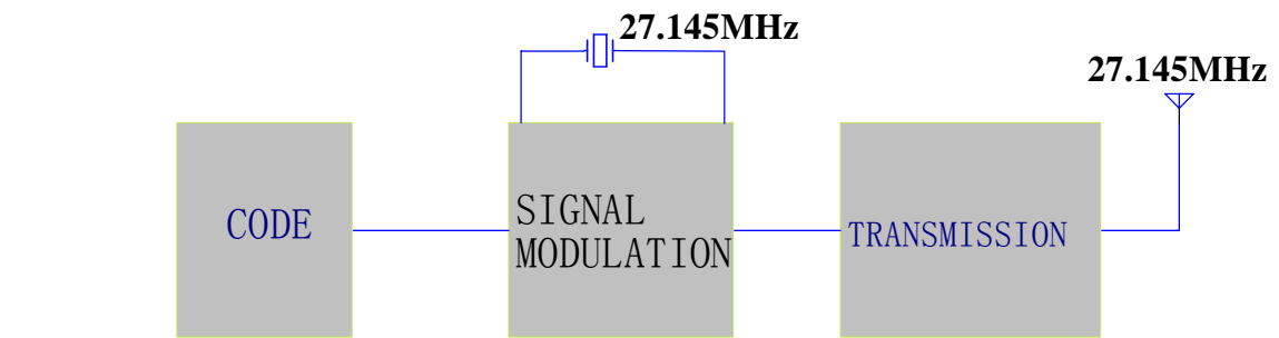
BLOCK DIAGRAM OF TRANSMISSION
