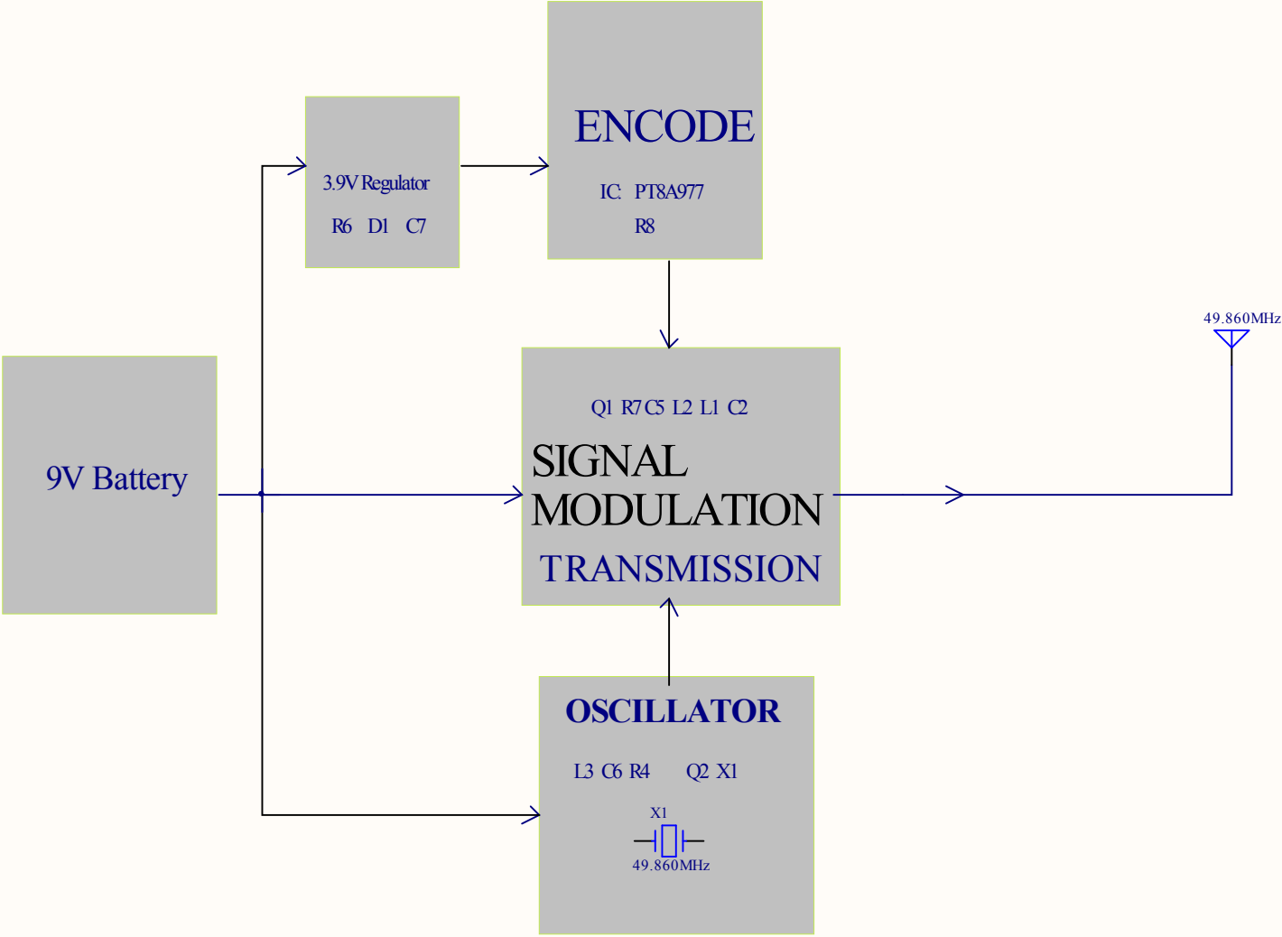
BLOCK DIAGRAM OF TRANSMISSION
