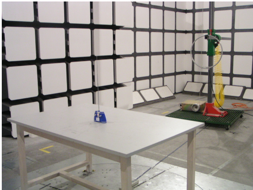
Below 30M Hz: Radiated Emission - Rear View
