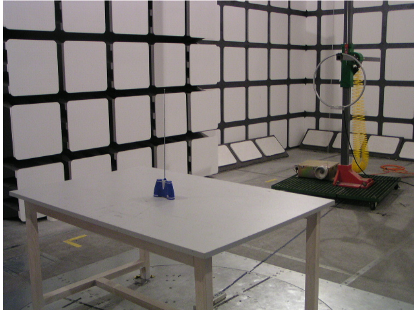
Below 30MHz: Radiated Emission - Front View
