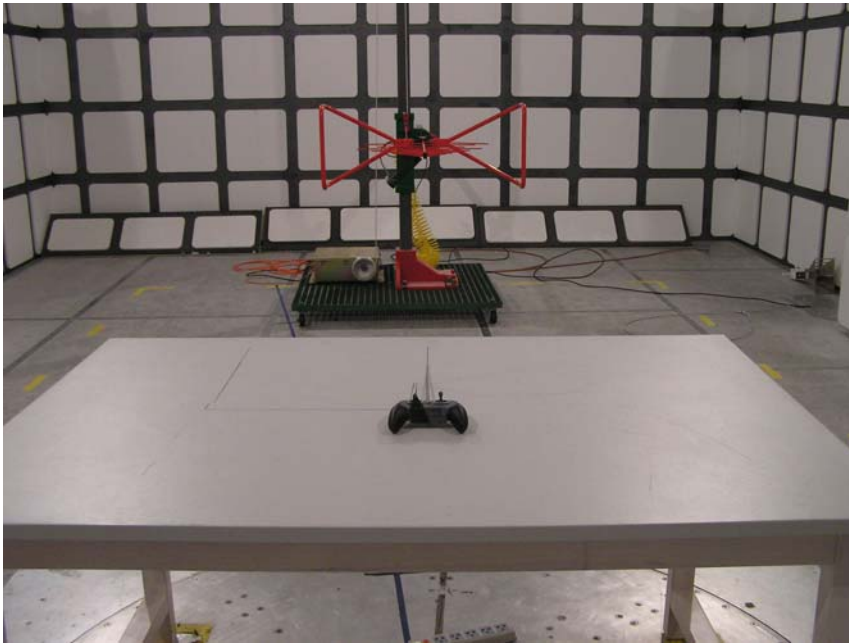
Radiated Emissions-Lie View (1)
