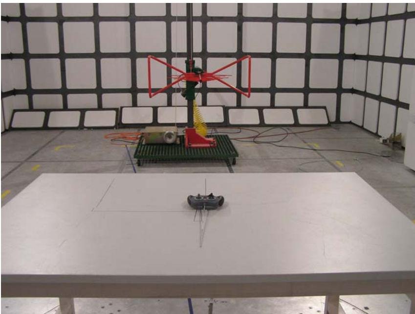
Radiated Emissions-Lie View (2)
