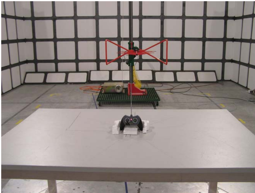
Radiated Emissions-Stand View
