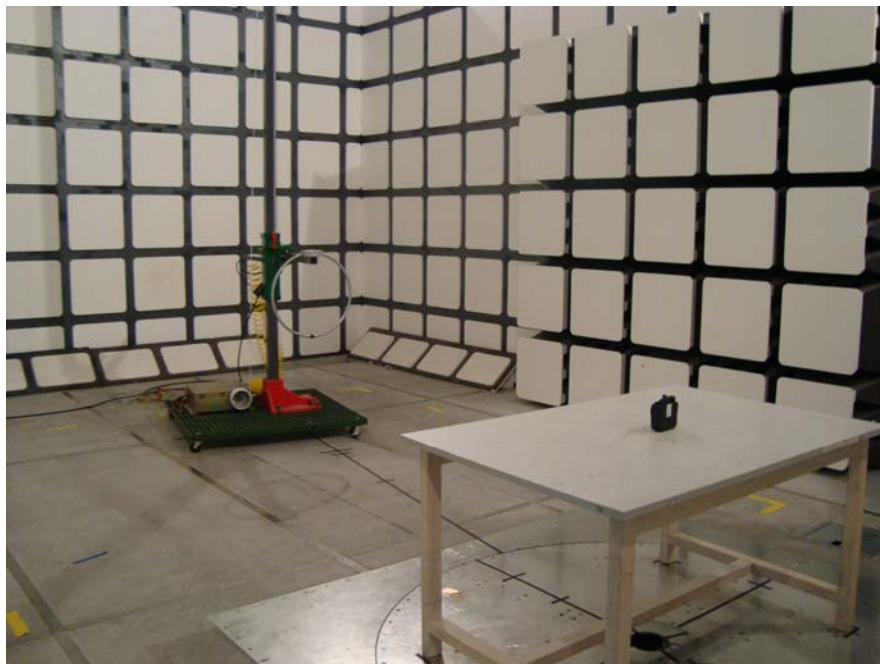
Radiated Emissions - Rear View (Fundamental)
