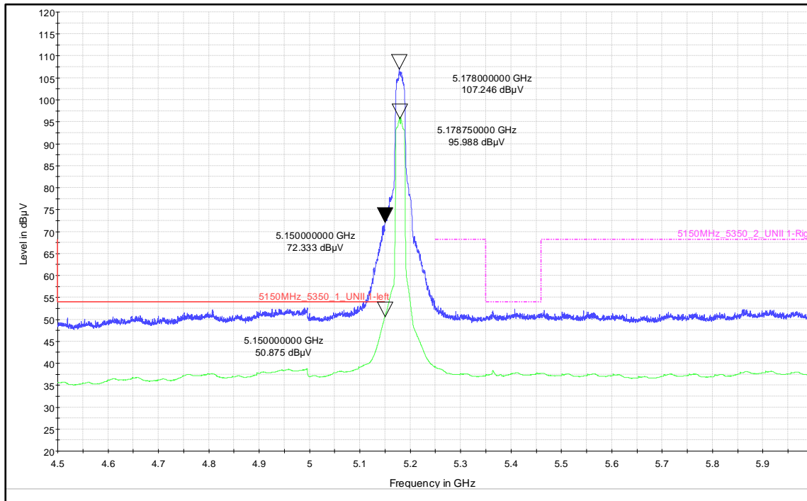
Fundamental Frequency
