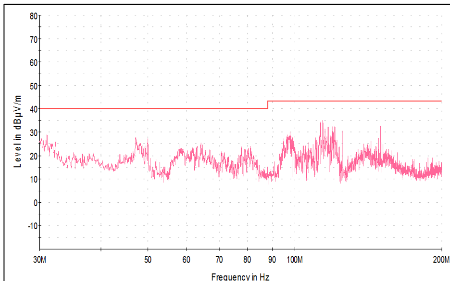
Polarization: Vertical
