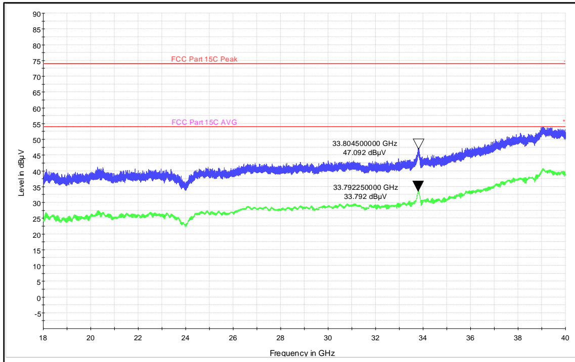
Frequency range:18GHz-40GHz
