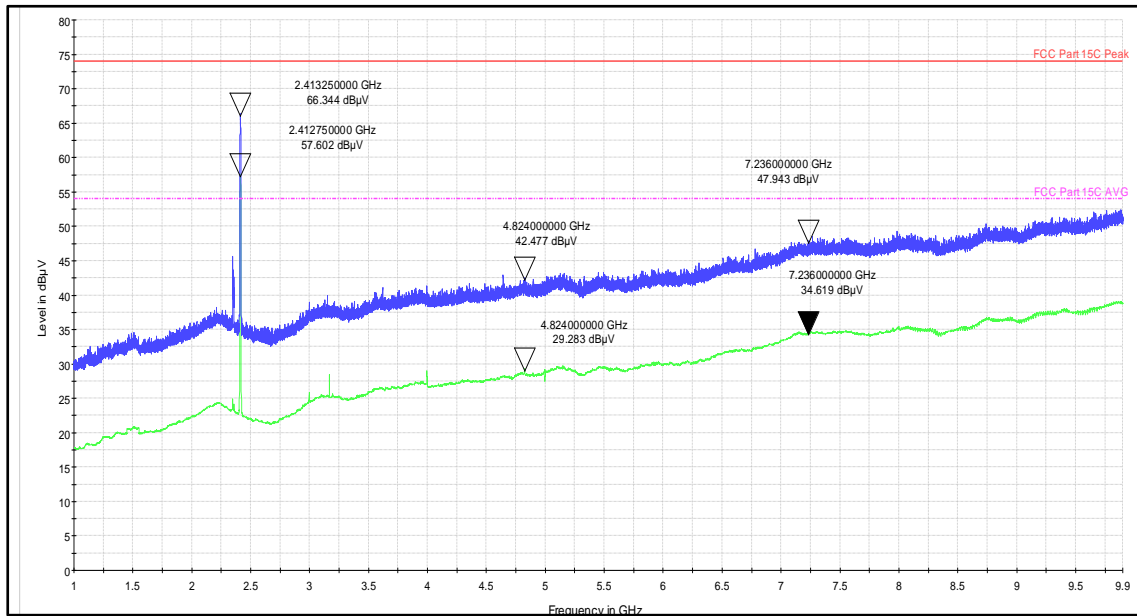
Frequency range:1GHz-9.9GHz
