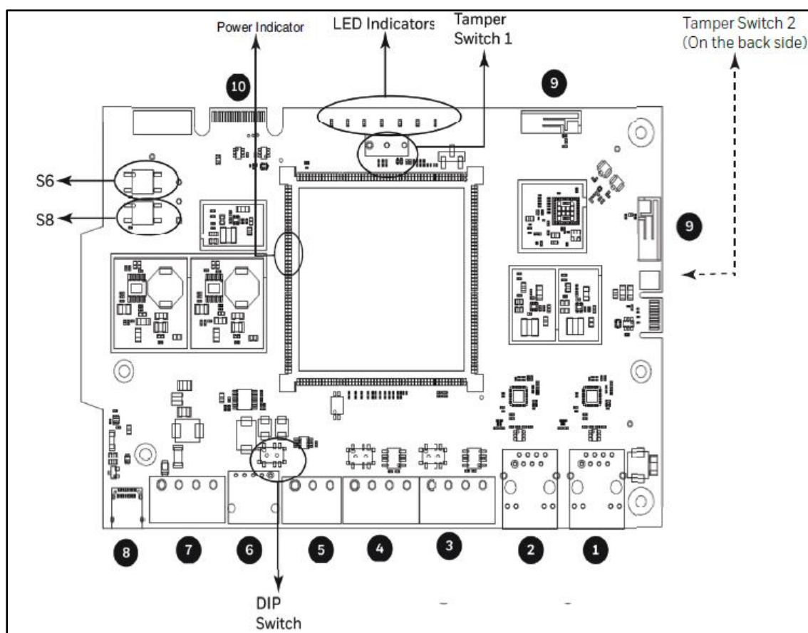
PCB Layout
