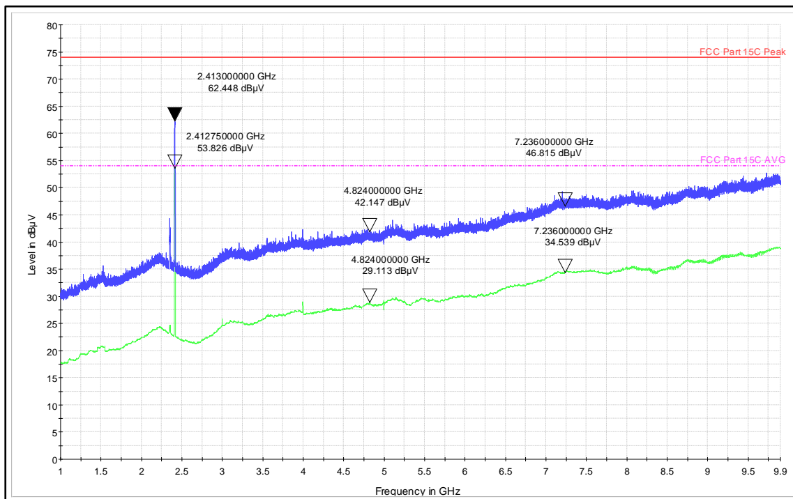
Frequency range:1GHz-9.9GHz
