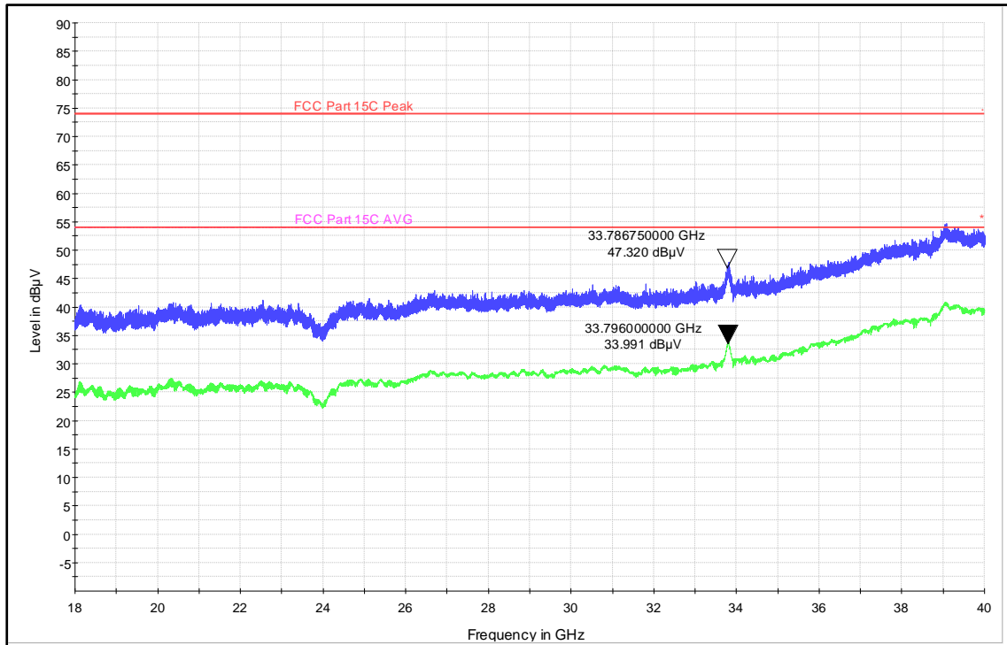
Frequency range:18GHz-40GHz
